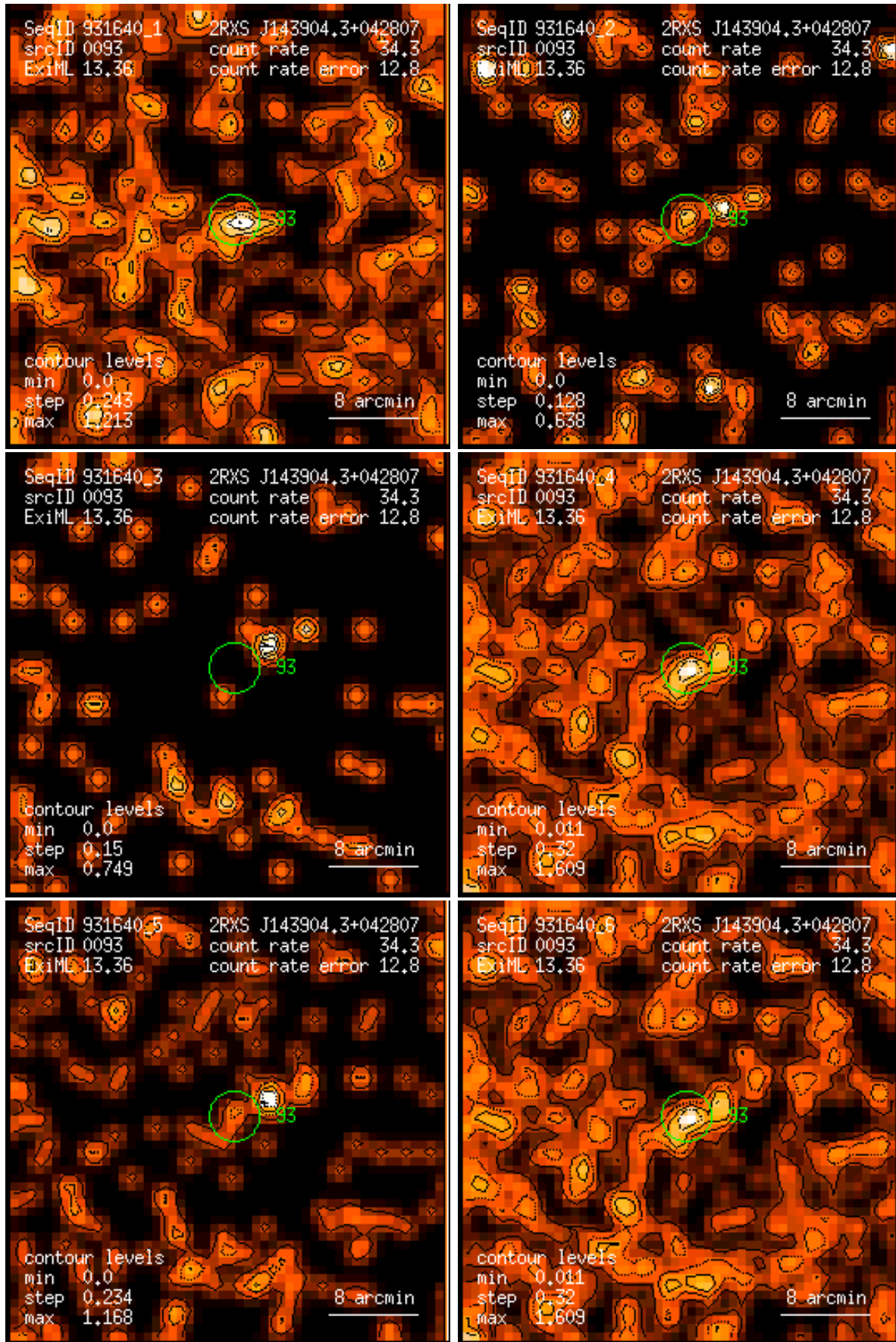
Figure 93: RASS 931640: detection 0093: band rate images, Gaussian filter: (1) PSPC channels 11 – 41, (2) 52 – 90, (3) 91 – 201, (4) 11 – 235, (5) 52 – 201, (6) 11 – 201. Broad band rates in counts/ks. Band rate contour levels in counts/ks/arcmin 2 .
