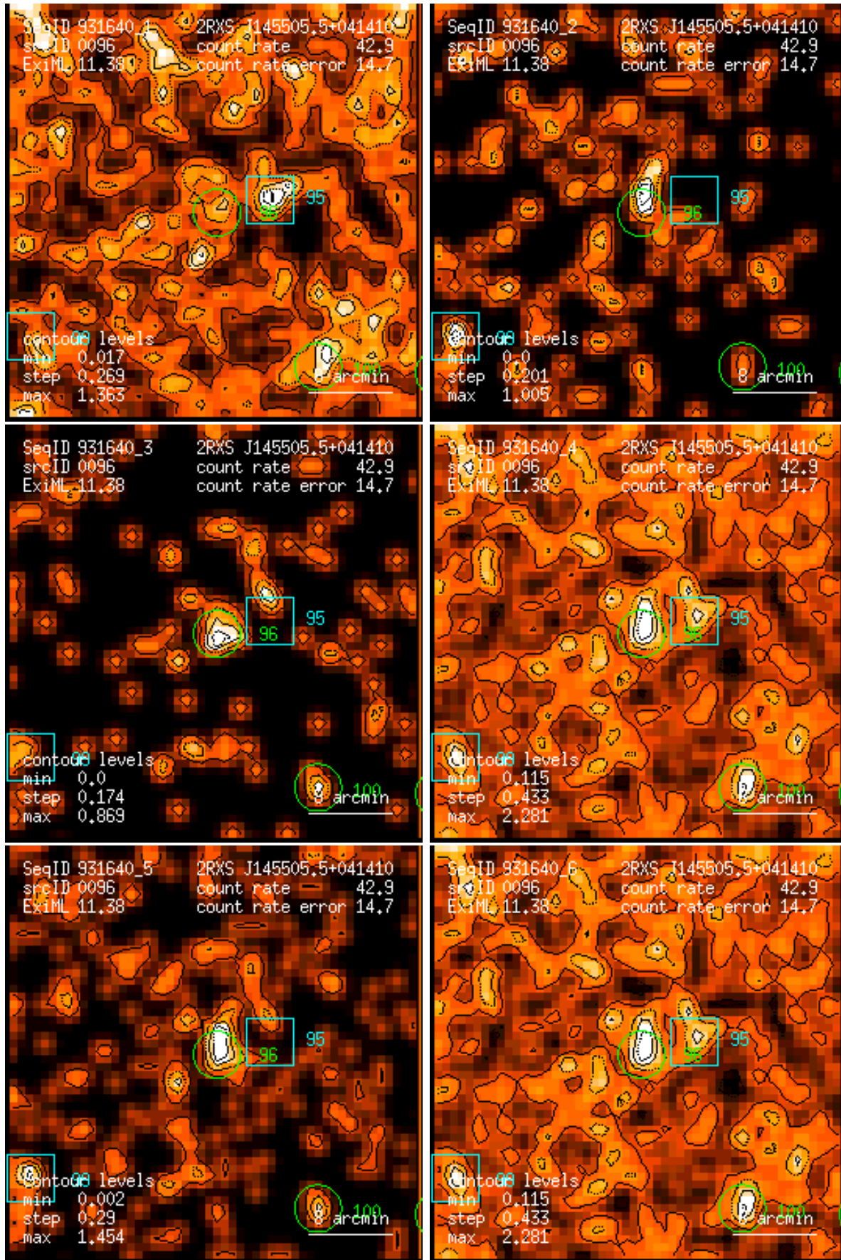
Figure 96: RASS 931640: detection 0096: band rate images, Gaussian filter: (1) PSPC channels 11 – 41, (2) 52 – 90, (3) 91 – 201, (4) 11 – 235, (5) 52 – 201, (6) 11 – 201. Broad band rates in counts/ks. Band rate contour levels in counts/ks/arcmin 2 .
