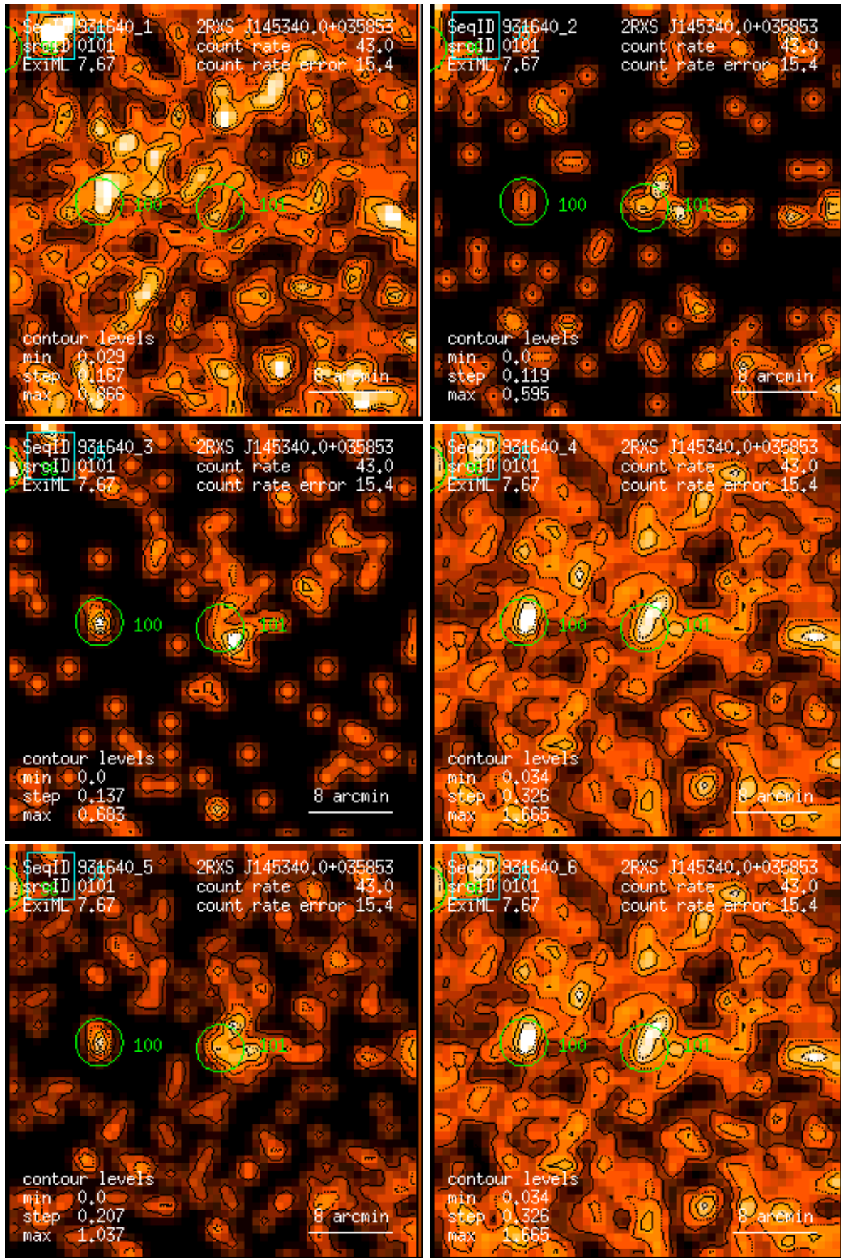
Figure 101: RASS 931640: detection 0101: band rate images, Gaussian filter: (1) PSPC channels 11 – 41, (2) 52 – 90, (3) 91 – 201, (4) 11 – 235, (5) 52 – 201, (6) 11 – 201. Broad band rates in counts/ks. Band rate contour levels in counts/ks/arcmin 2 .
