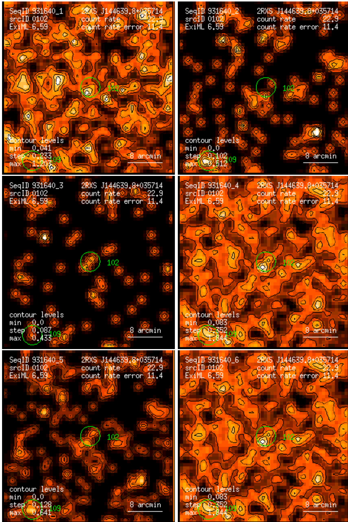
Figure 102: RASS 931640: detection 0102: band rate images, Gaussian filter: (1) PSPC channels 11 – 41, (2) 52 – 90, (3) 91 – 201, (4) 11 – 235, (5) 52 – 201, (6) 11 – 201. Broad band rates in counts/ks. Band rate contour levels in counts/ks/arcmin 2 .
