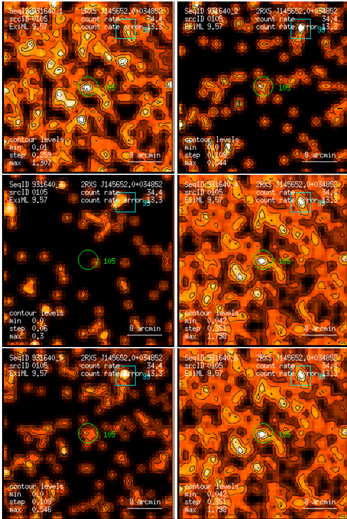
Figure 105: RASS 931640: detection 0105: band rate images, Gaussian filter: (1) PSPC channels 11 – 41, (2) 52 – 90, (3) 91 – 201, (4) 11 – 235, (5) 52 – 201, (6) 11 – 201. Broad band rates in counts/ks. Band rate contour levels in counts/ks/arcmin 2 .
