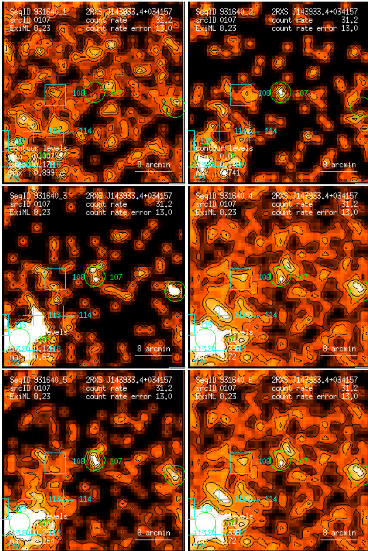
Figure 107: RASS 931640: detection 0107: band rate images, Gaussian filter: (1) PSPC channels 11 – 41, (2) 52 – 90, (3) 91 – 201, (4) 11 – 235, (5) 52 – 201, (6) 11 – 201. Broad band rates in counts/ks. Band rate contour levels in counts/ks/arcmin 2 .
