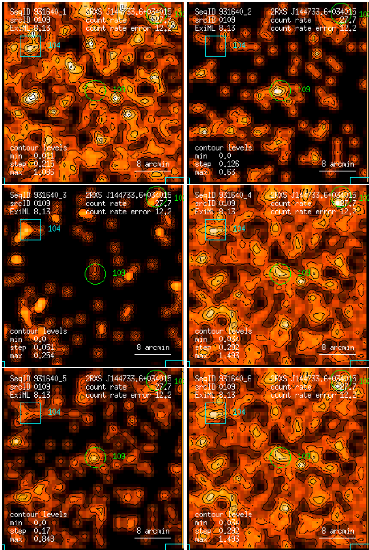
Figure 109: RASS 931640: detection 0109: band rate images, Gaussian filter: (1) PSPC channels 11 – 41, (2) 52 – 90, (3) 91 – 201, (4) 11 – 235, (5) 52 – 201, (6) 11 – 201. Broad band rates in counts/ks. Band rate contour levels in counts/ks/arcmin 2 .
