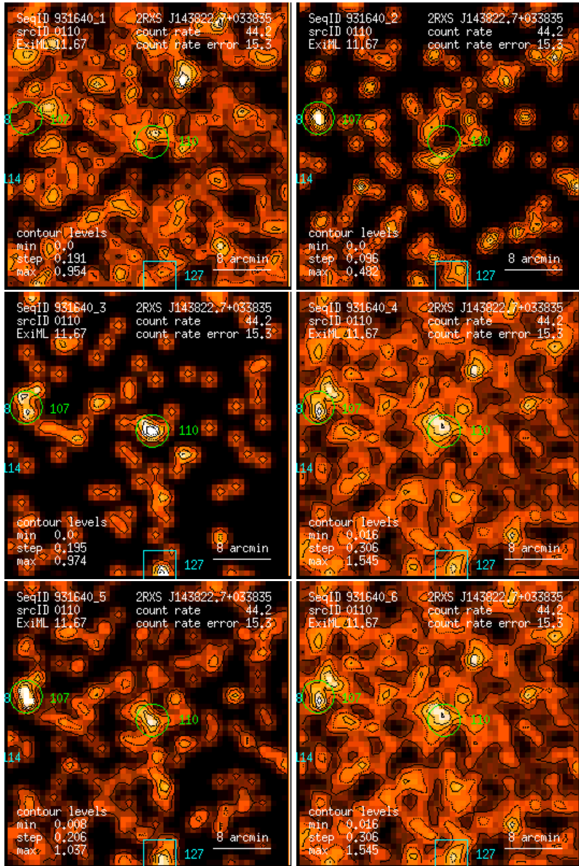
Figure 110: RASS 931640: detection 0110: band rate images, Gaussian filter: (1) PSPC channels 11 – 41, (2) 52 – 90, (3) 91 – 201, (4) 11 – 235, (5) 52 – 201, (6) 11 – 201. Broad band rates in counts/ks. Band rate contour levels in counts/ks/arcmin 2 .
