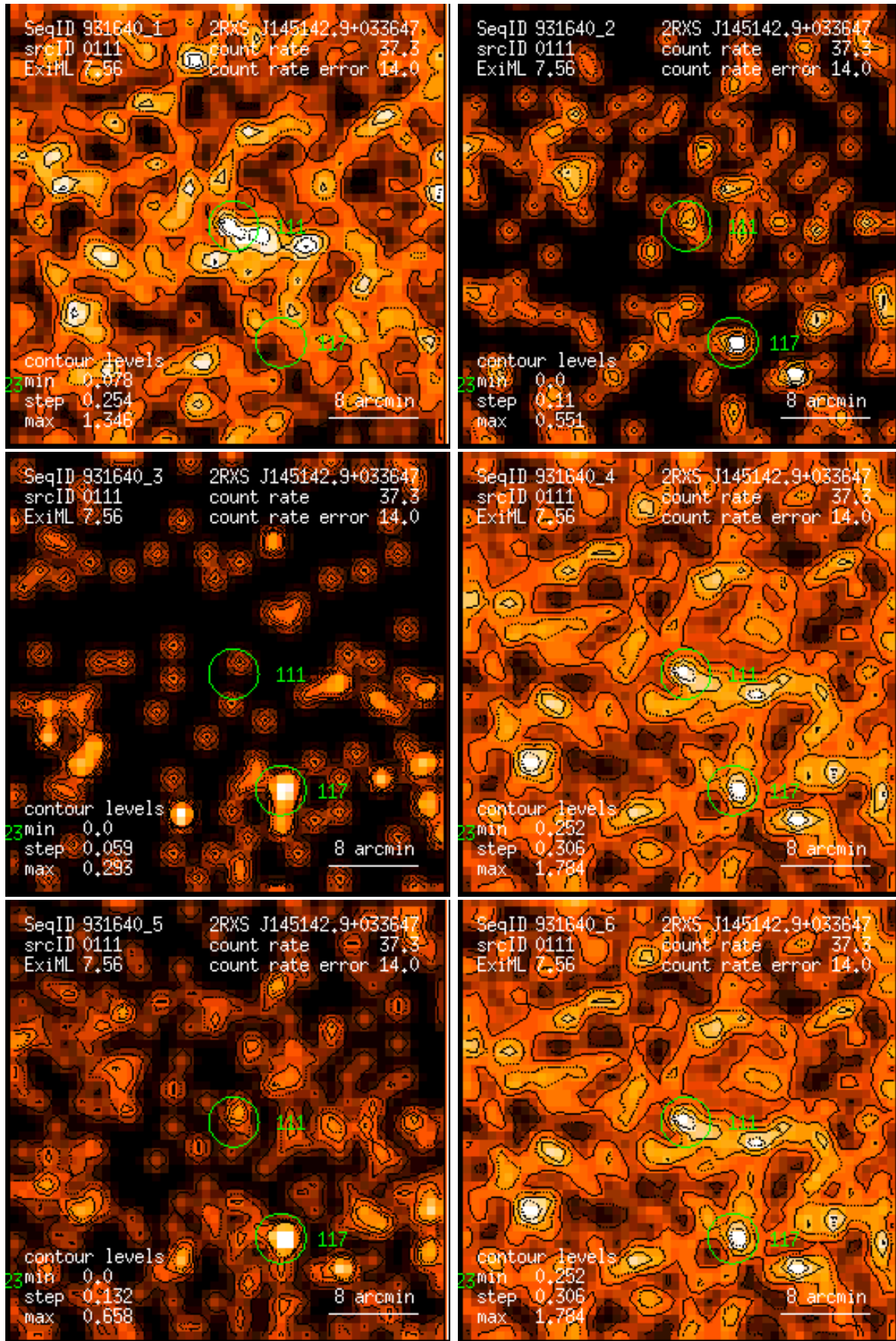
Figure 111: RASS 931640: detection 0111: band rate images, Gaussian filter: (1) PSPC channels 11 – 41, (2) 52 – 90, (3) 91 – 201, (4) 11 – 235, (5) 52 – 201, (6) 11 – 201. Broad band rates in counts/ks. Band rate contour levels in counts/ks/arcmin 2 .
