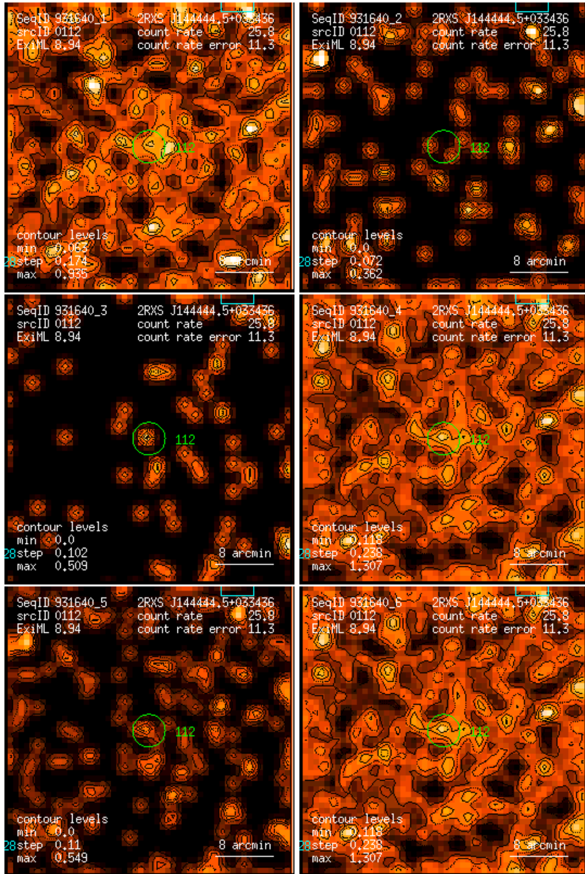
Figure 112: RASS 931640: detection 0112: band rate images, Gaussian filter: (1) PSPC channels 11 – 41, (2) 52 – 90, (3) 91 – 201, (4) 11 – 235, (5) 52 – 201, (6) 11 – 201. Broad band rates in counts/ks. Band rate contour levels in counts/ks/arcmin 2 .
