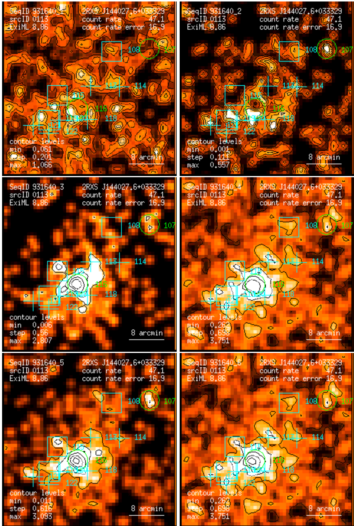
Figure 113: RASS 931640: detection 0113: band rate images, Gaussian filter: (1) PSPC channels 11 – 41, (2) 52 – 90, (3) 91 – 201, (4) 11 – 235, (5) 52 – 201, (6) 11 – 201. Broad band rates in counts/ks. Band rate contour levels in counts/ks/arcmin 2 .
