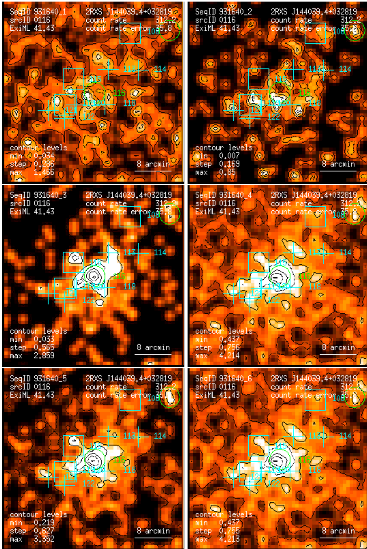
Figure 116: RASS 931640: detection 0116: band rate images, Gaussian filter: (1) PSPC channels 11 – 41, (2) 52 – 90, (3) 91 – 201, (4) 11 – 235, (5) 52 – 201, (6) 11 – 201. Broad band rates in counts/ks. Band rate contour levels in counts/ks/arcmin 2 .
