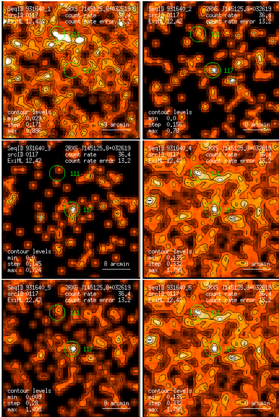
Figure 117: RASS 931640: detection 0117: band rate images, Gaussian filter: (1) PSPC channels 11 – 41, (2) 52 – 90, (3) 91 – 201, (4) 11 – 235, (5) 52 – 201, (6) 11 – 201. Broad band rates in counts/ks. Band rate contour levels in counts/ks/arcmin 2 .
