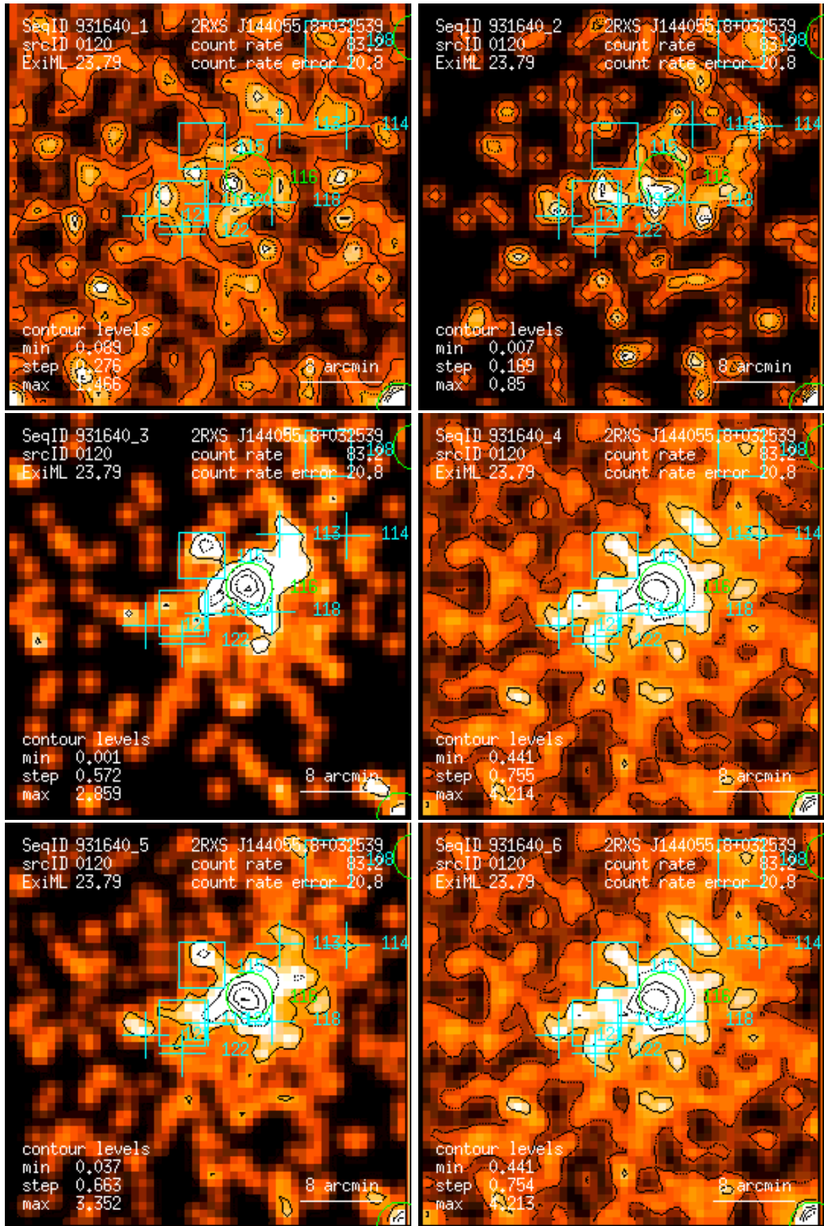
Figure 120: RASS 931640: detection 0120: band rate images, Gaussian filter: (1) PSPC channels 11 – 41, (2) 52 – 90, (3) 91 – 201, (4) 11 – 235, (5) 52 – 201, (6) 11 – 201. Broad band rates in counts/ks. Band rate contour levels in counts/ks/arcmin 2 .
