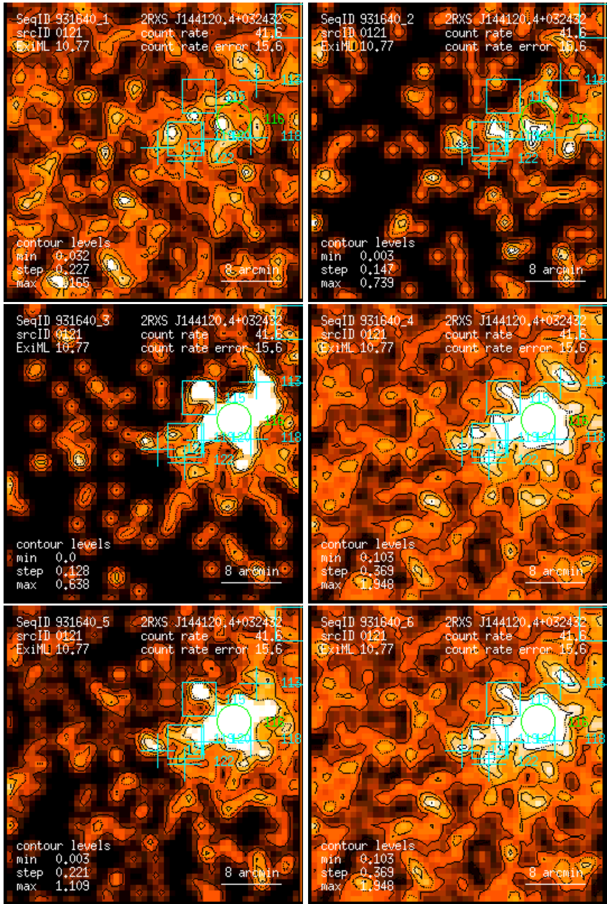
Figure 121: RASS 931640: detection 0121: band rate images, Gaussian filter: (1) PSPC channels 11 – 41, (2) 52 – 90, (3) 91 – 201, (4) 11 – 235, (5) 52 – 201, (6) 11 – 201. Broad band rates in counts/ks. Band rate contour levels in counts/ks/arcmin 2 .
