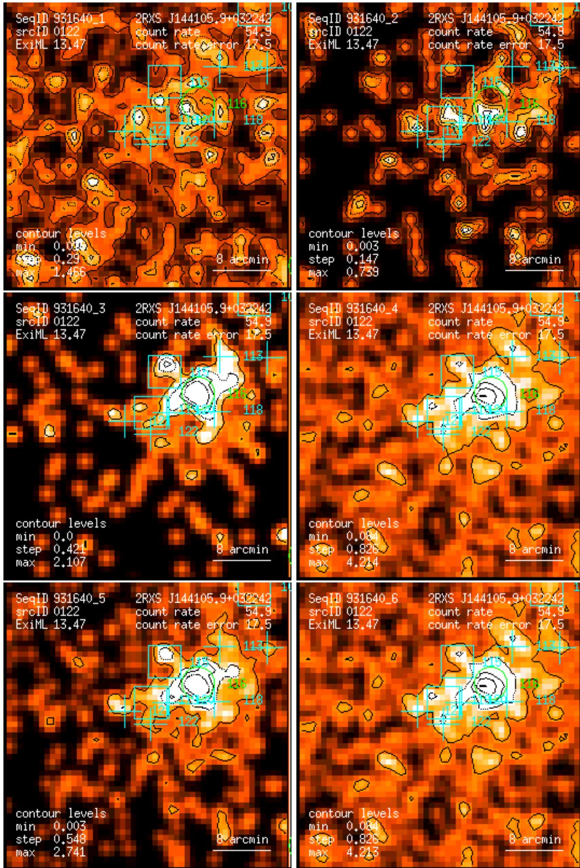
Figure 122: RASS 931640: detection 0122: band rate images, Gaussian filter: (1) PSPC channels 11 – 41, (2) 52 – 90, (3) 91 – 201, (4) 11 – 235, (5) 52 – 201, (6) 11 – 201. Broad band rates in counts/ks. Band rate contour levels in counts/ks/arcmin 2 .
