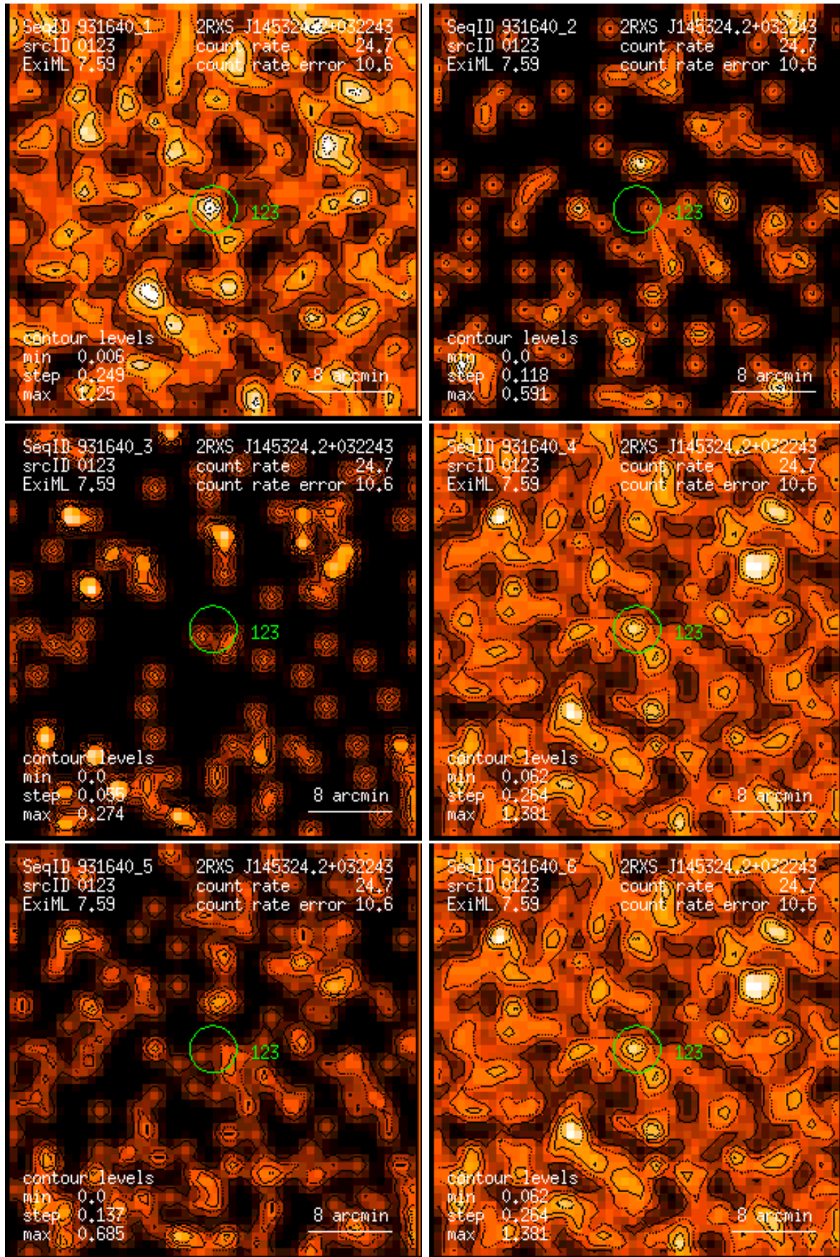
Figure 123: RASS 931640: detection 0123: band rate images, Gaussian filter: (1) PSPC channels 11 – 41, (2) 52 – 90, (3) 91 – 201, (4) 11 – 235, (5) 52 – 201, (6) 11 – 201. Broad band rates in counts/ks. Band rate contour levels in counts/ks/arcmin 2 .
