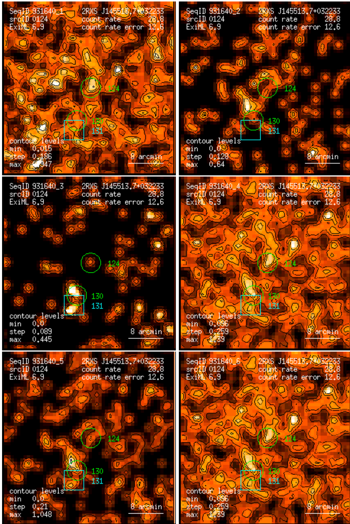
Figure 124: RASS 931640: detection 0124: band rate images, Gaussian filter: (1) PSPC channels 11 – 41, (2) 52 – 90, (3) 91 – 201, (4) 11 – 235, (5) 52 – 201, (6) 11 – 201. Broad band rates in counts/ks. Band rate contour levels in counts/ks/arcmin 2 .
