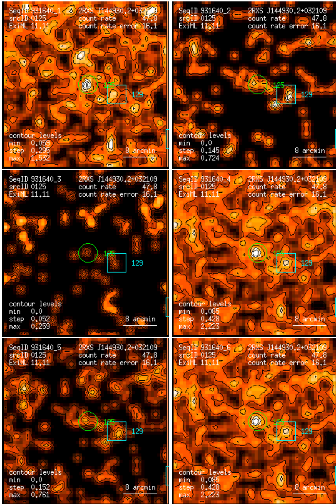
Figure 125: RASS 931640: detection 0125: band rate images, Gaussian filter: (1) PSPC channels 11 – 41, (2) 52 – 90, (3) 91 – 201, (4) 11 – 235, (5) 52 – 201, (6) 11 – 201. Broad band rates in counts/ks. Band rate contour levels in counts/ks/arcmin 2 .
