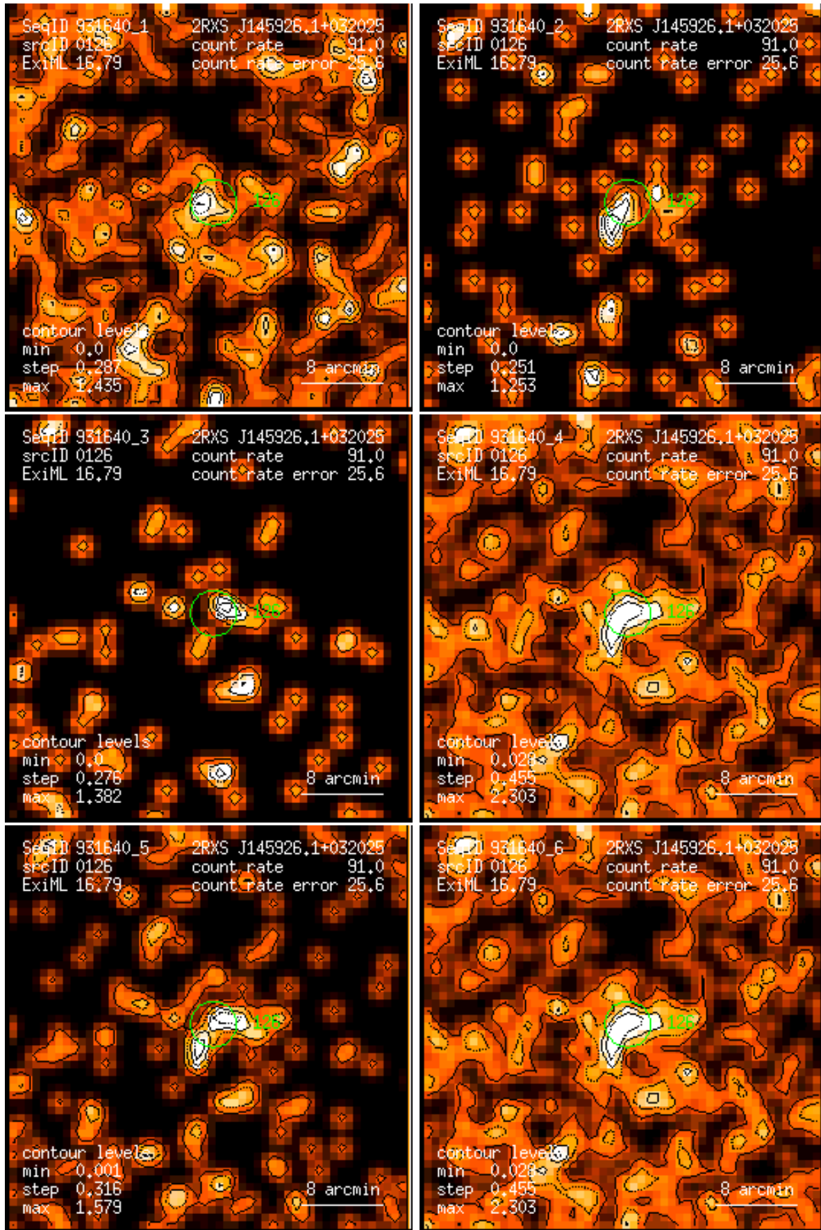
Figure 126: RASS 931640: detection 0126: band rate images, Gaussian filter: (1) PSPC channels 11 – 41, (2) 52 – 90, (3) 91 – 201, (4) 11 – 235, (5) 52 – 201, (6) 11 – 201. Broad band rates in counts/ks. Band rate contour levels in counts/ks/arcmin 2 .
