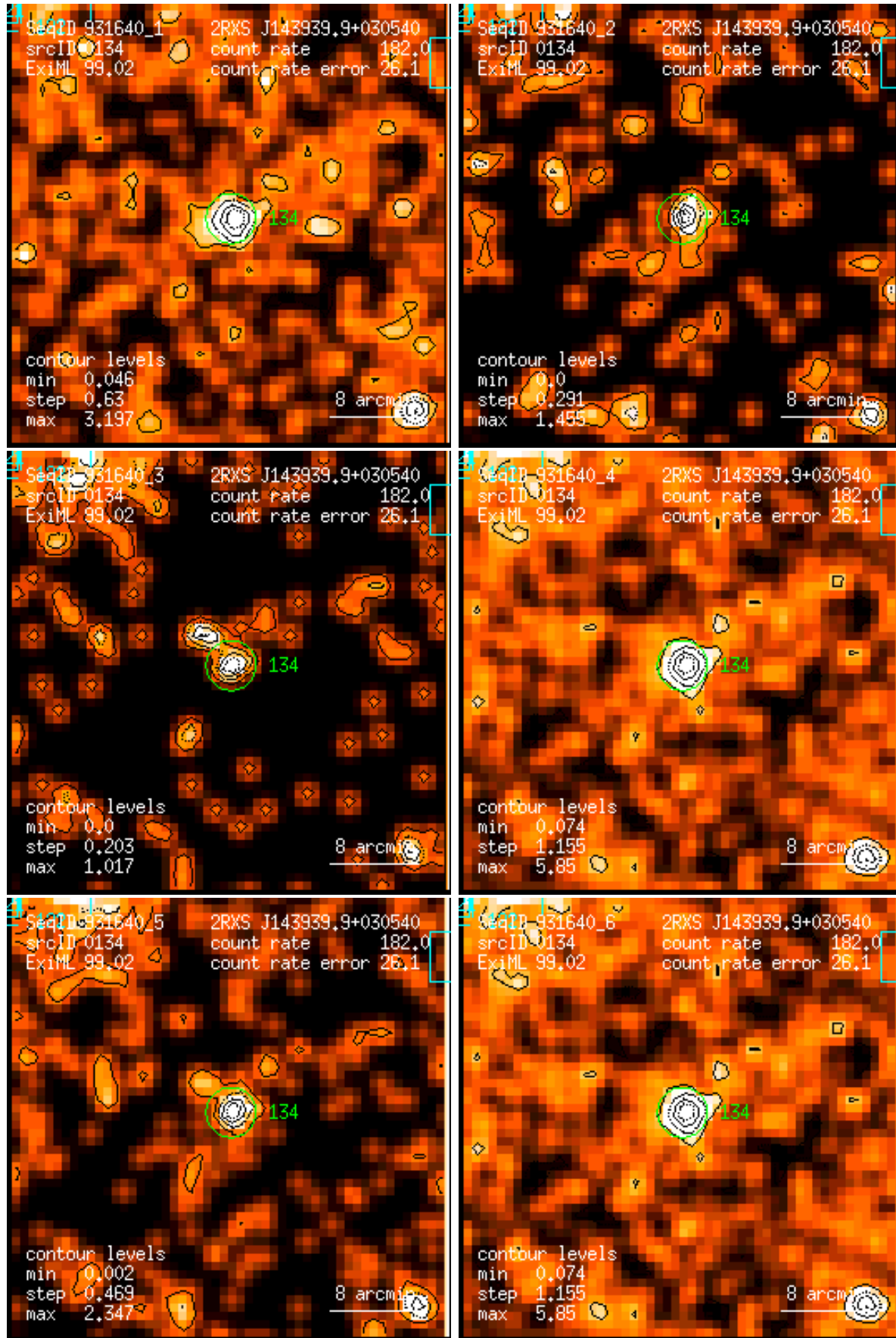
Figure 134: RASS 931640: detection 0134: band rate images, Gaussian filter: (1) PSPC channels 11 – 41, (2) 52 – 90, (3) 91 – 201, (4) 11 – 235, (5) 52 – 201, (6) 11 – 201. Broad band rates in counts/ks. Band rate contour levels in counts/ks/arcmin 2 .
