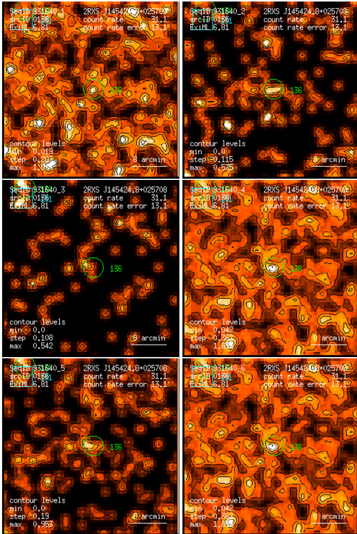
Figure 136: RASS 931640: detection 0136: band rate images, Gaussian filter: (1) PSPC channels 11 – 41, (2) 52 – 90, (3) 91 – 201, (4) 11 – 235, (5) 52 – 201, (6) 11 – 201. Broad band rates in counts/ks. Band rate contour levels in counts/ks/arcmin 2 .
