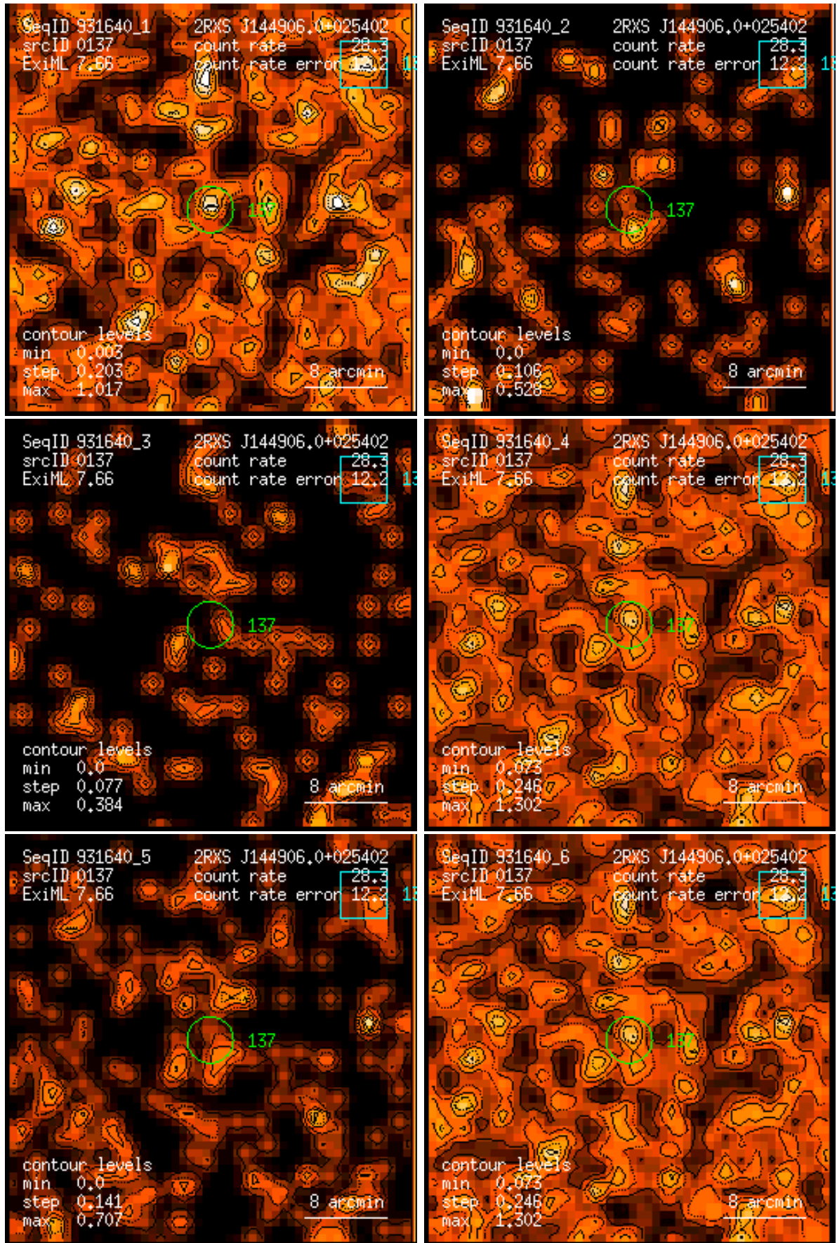
Figure 137: RASS 931640: detection 0137: band rate images, Gaussian filter: (1) PSPC channels 11 – 41, (2) 52 – 90, (3) 91 – 201, (4) 11 – 235, (5) 52 – 201, (6) 11 – 201. Broad band rates in counts/ks. Band rate contour levels in counts/ks/arcmin 2 .
