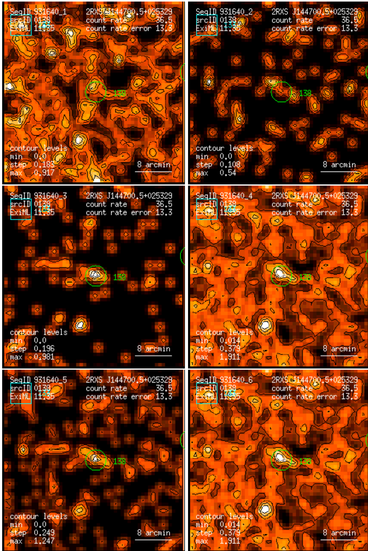
Figure 138: RASS 931640: detection 0138: band rate images, Gaussian filter: (1) PSPC channels 11 – 41, (2) 52 – 90, (3) 91 – 201, (4) 11 – 235, (5) 52 – 201, (6) 11 – 201. Broad band rates in counts/ks. Band rate contour levels in counts/ks/arcmin 2 .
