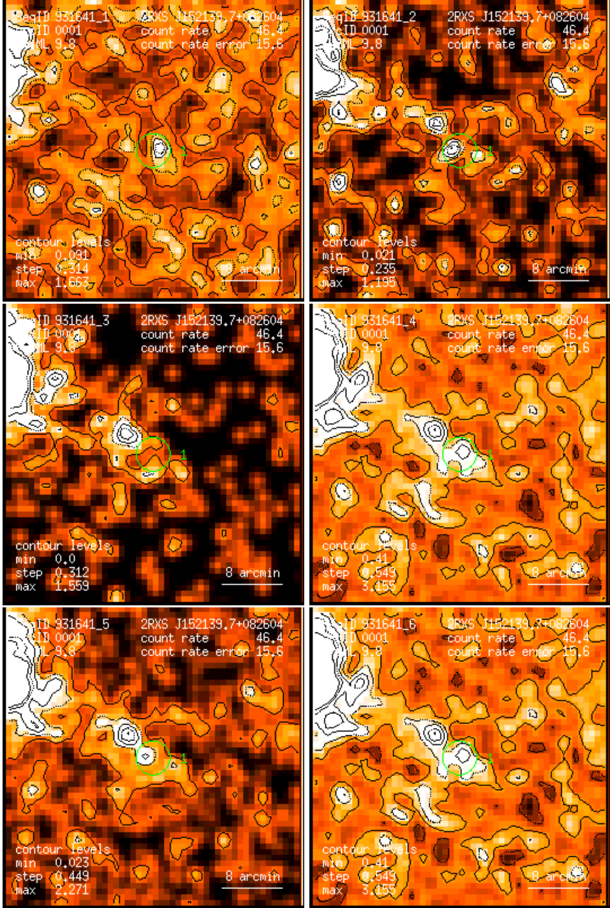
Figure 1: RASS 931641: detection 0001: band rate images, Gaussian filter: (1) PSPC channels 11 – 41, (2) 52 – 90, (3) 91 – 201, (4) 11 – 235, (5) 52 – 201, (6) 11 – 201. Broad band rates in counts/ks. Band rate contour levels in counts/ks/arcmin 2 .
