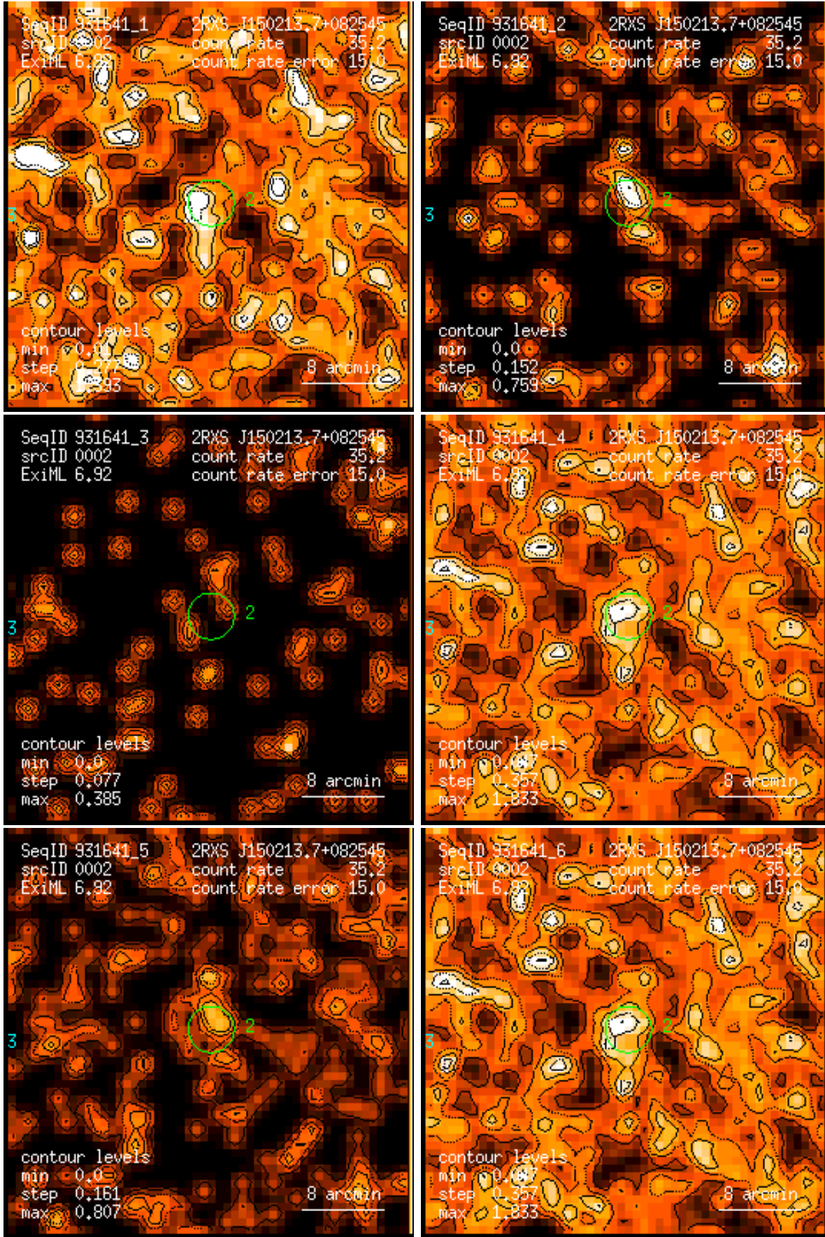
Figure 2: RASS 931641: detection 0002: band rate images, Gaussian filter: (1) PSPC channels 11 – 41, (2) 52 – 90, (3) 91 – 201, (4) 11 – 235, (5) 52 – 201, (6) 11 – 201. Broad band rates in counts/ks. Band rate contour levels in counts/ks/arcmin 2 .
