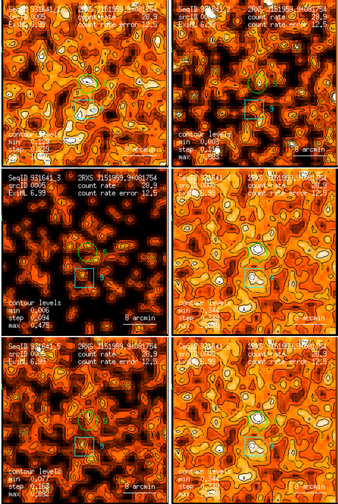
Figure 5: RASS 931641: detection 0005: band rate images, Gaussian filter: (1) PSPC channels 11 – 41, (2) 52 – 90, (3) 91 – 201, (4) 11 – 235, (5) 52 – 201, (6) 11 – 201. Broad band rates in counts/ks. Band rate contour levels in counts/ks/arcmin 2 .
