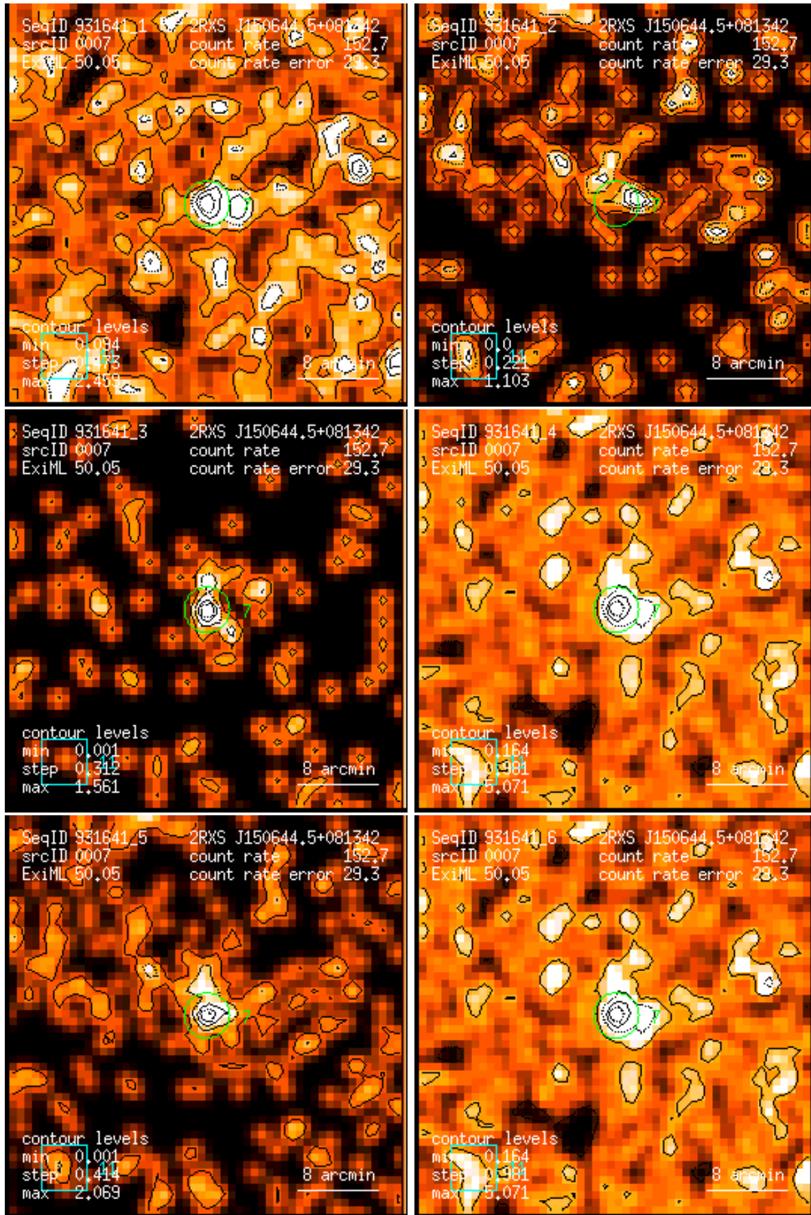
Figure 7: RASS 931641: detection 0007: band rate images, Gaussian filter: (1) PSPC channels 11 – 41, (2) 52 – 90, (3) 91 – 201, (4) 11 – 235, (5) 52 – 201, (6) 11 – 201. Broad band rates in counts/ks. Band rate contour levels in counts/ks/arcmin 2 .
