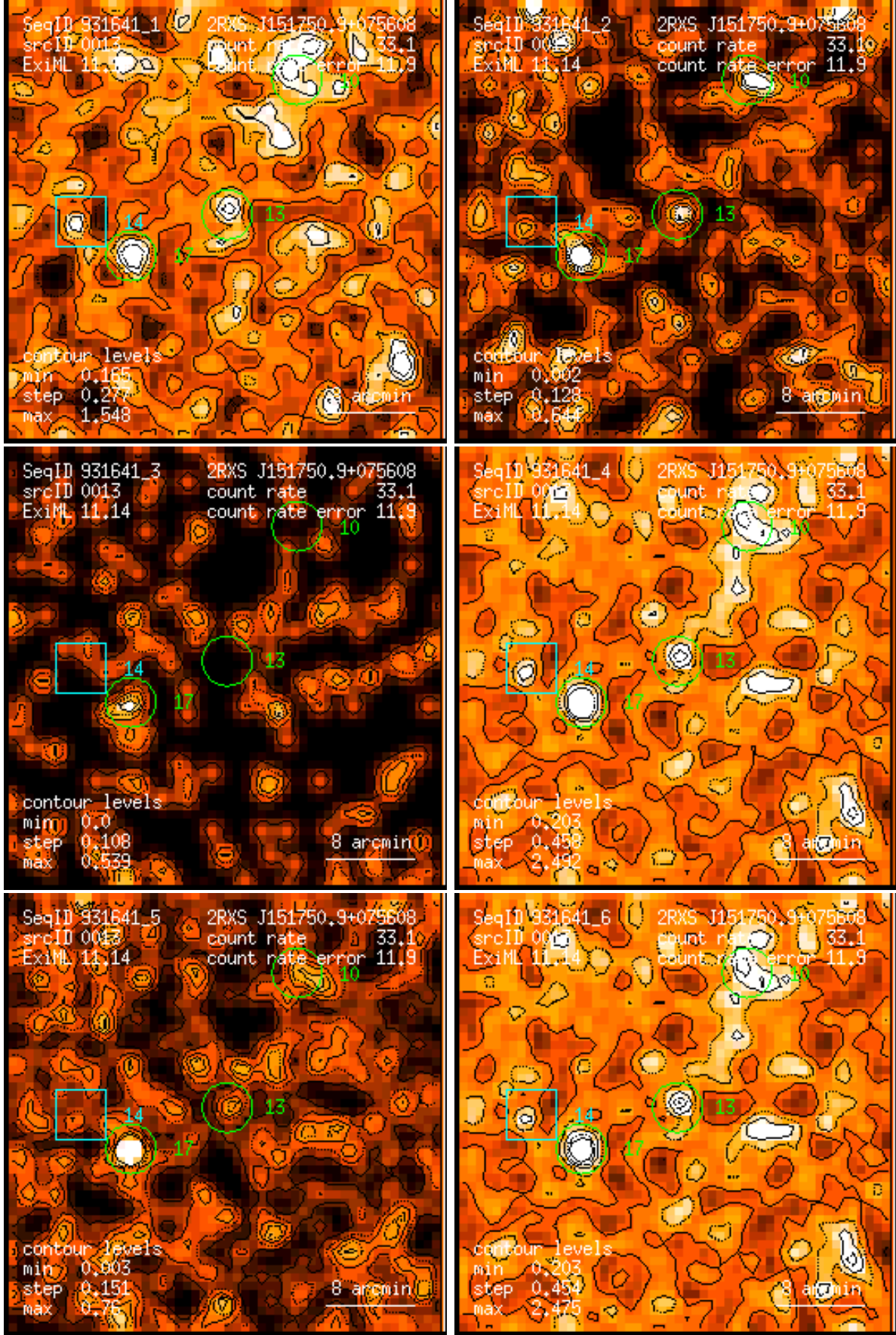
Figure 13: RASS 931641: detection 0013: band rate images, Gaussian filter: (1) PSPC channels 11 – 41, (2) 52 – 90, (3) 91 – 201, (4) 11 – 235, (5) 52 – 201, (6) 11 – 201. Broad band rates in counts/ks. Band rate contour levels in counts/ks/arcmin 2 .
