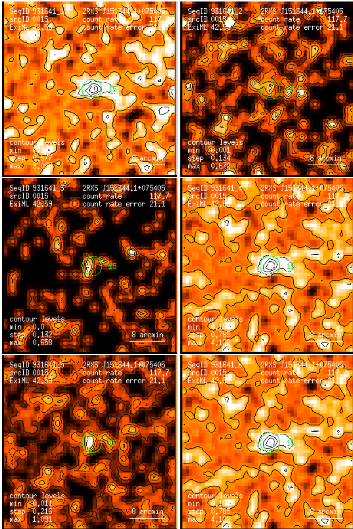
Figure 15: RASS 931641: detection 0015: band rate images, Gaussian filter: (1) PSPC channels 11 – 41, (2) 52 – 90, (3) 91 – 201, (4) 11 – 235, (5) 52 – 201, (6) 11 – 201. Broad band rates in counts/ks. Band rate contour levels in counts/ks/arcmin 2 .
