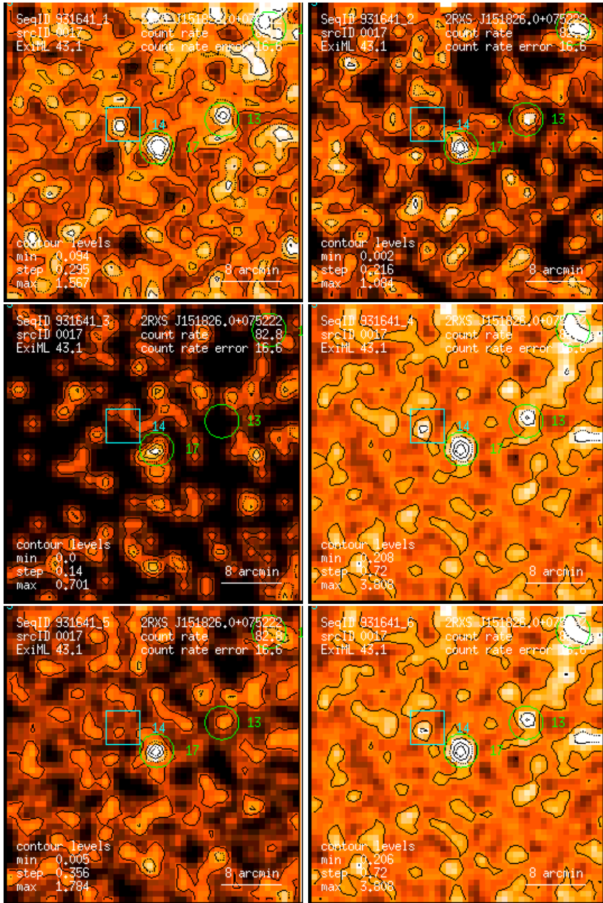
Figure 17: RASS 931641: detection 0017: band rate images, Gaussian filter: (1) PSPC channels 11 – 41, (2) 52 – 90, (3) 91 – 201, (4) 11 – 235, (5) 52 – 201, (6) 11 – 201. Broad band rates in counts/ks. Band rate contour levels in counts/ks/arcmin 2 .
