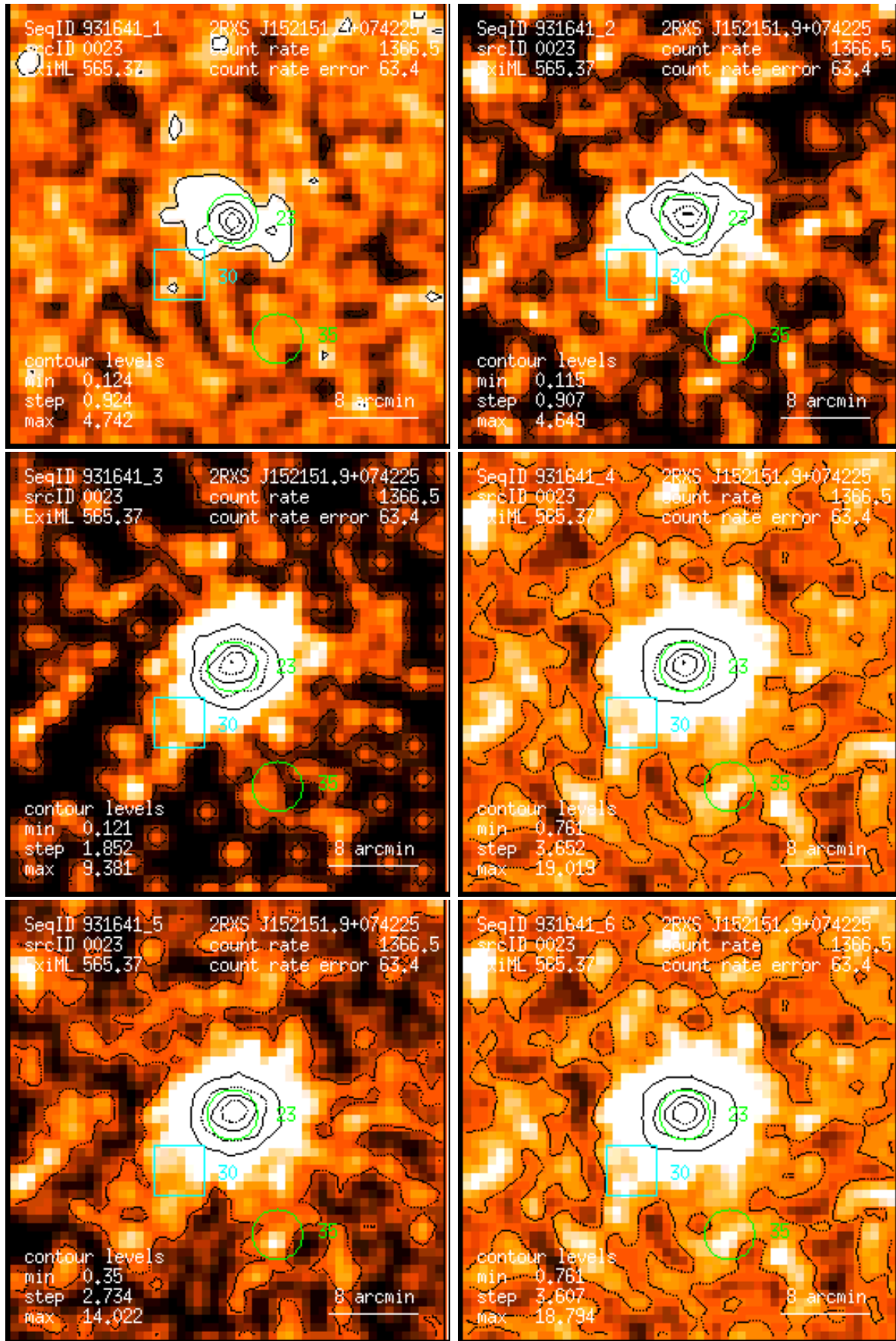
Figure 23: RASS 931641: detection 0023: band rate images, Gaussian filter: (1) PSPC channels 11 – 41, (2) 52 – 90, (3) 91 – 201, (4) 11 – 235, (5) 52 – 201, (6) 11 – 201. Broad band rates in counts/ks. Band rate contour levels in counts/ks/arcmin 2 .
