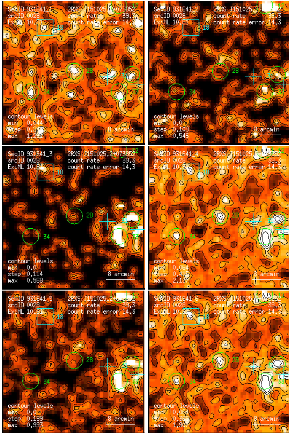
Figure 28: RASS 931641: detection 0028: band rate images, Gaussian filter: (1) PSPC channels 11 – 41, (2) 52 – 90, (3) 91 – 201, (4) 11 – 235, (5) 52 – 201, (6) 11 – 201. Broad band rates in counts/ks. Band rate contour levels in counts/ks/arcmin 2 .
