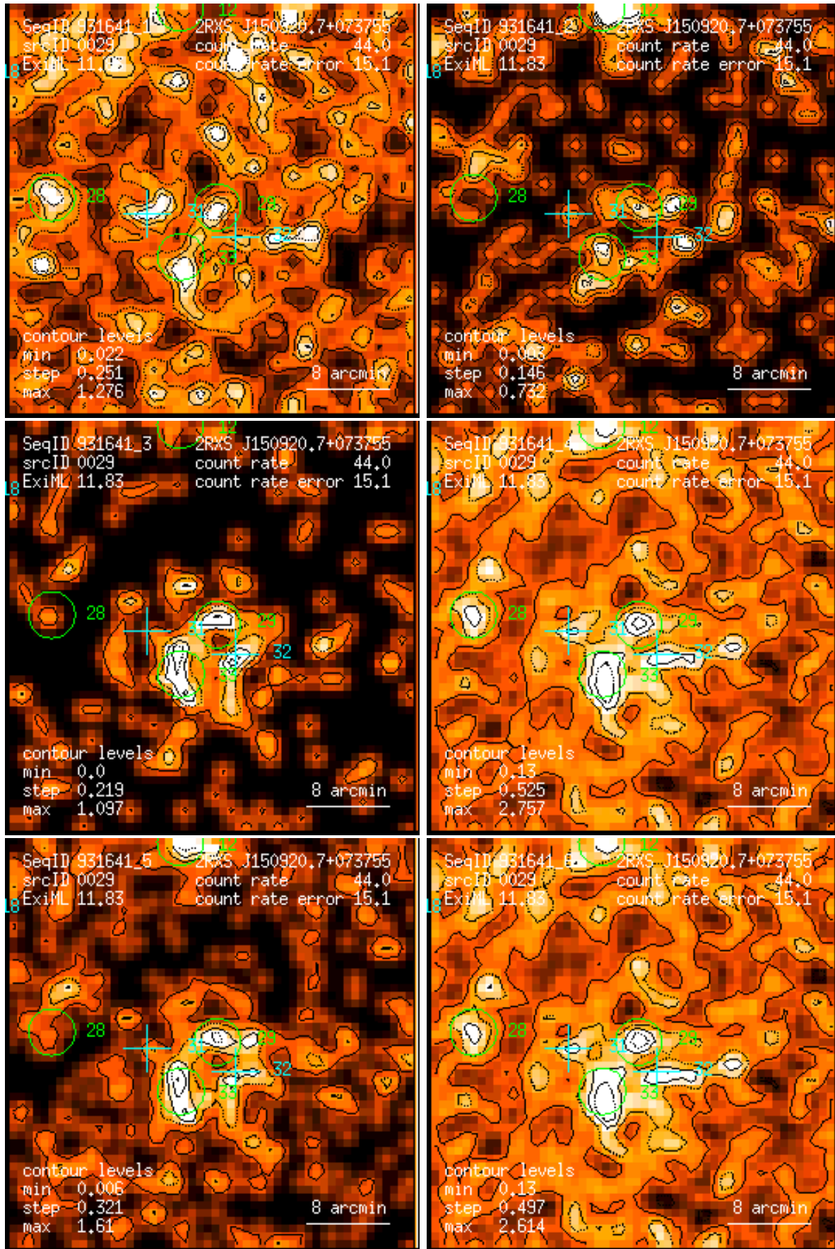
Figure 29: RASS 931641: detection 0029: band rate images, Gaussian filter: (1) PSPC channels 11 – 41, (2) 52 – 90, (3) 91 – 201, (4) 11 – 235, (5) 52 – 201, (6) 11 – 201. Broad band rates in counts/ks. Band rate contour levels in counts/ks/arcmin 2 .
