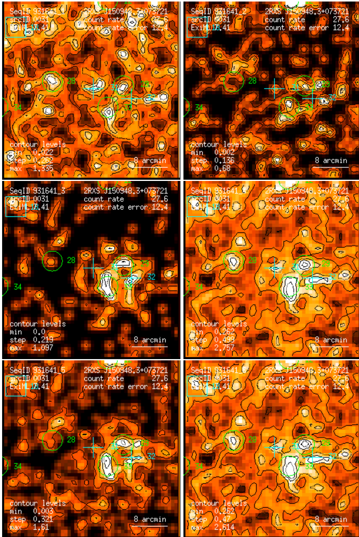
Figure 31: RASS 931641: detection 0031: band rate images, Gaussian filter: (1) PSPC channels 11 – 41, (2) 52 – 90, (3) 91 – 201, (4) 11 – 235, (5) 52 – 201, (6) 11 – 201. Broad band rates in counts/ks. Band rate contour levels in counts/ks/arcmin 2 .
