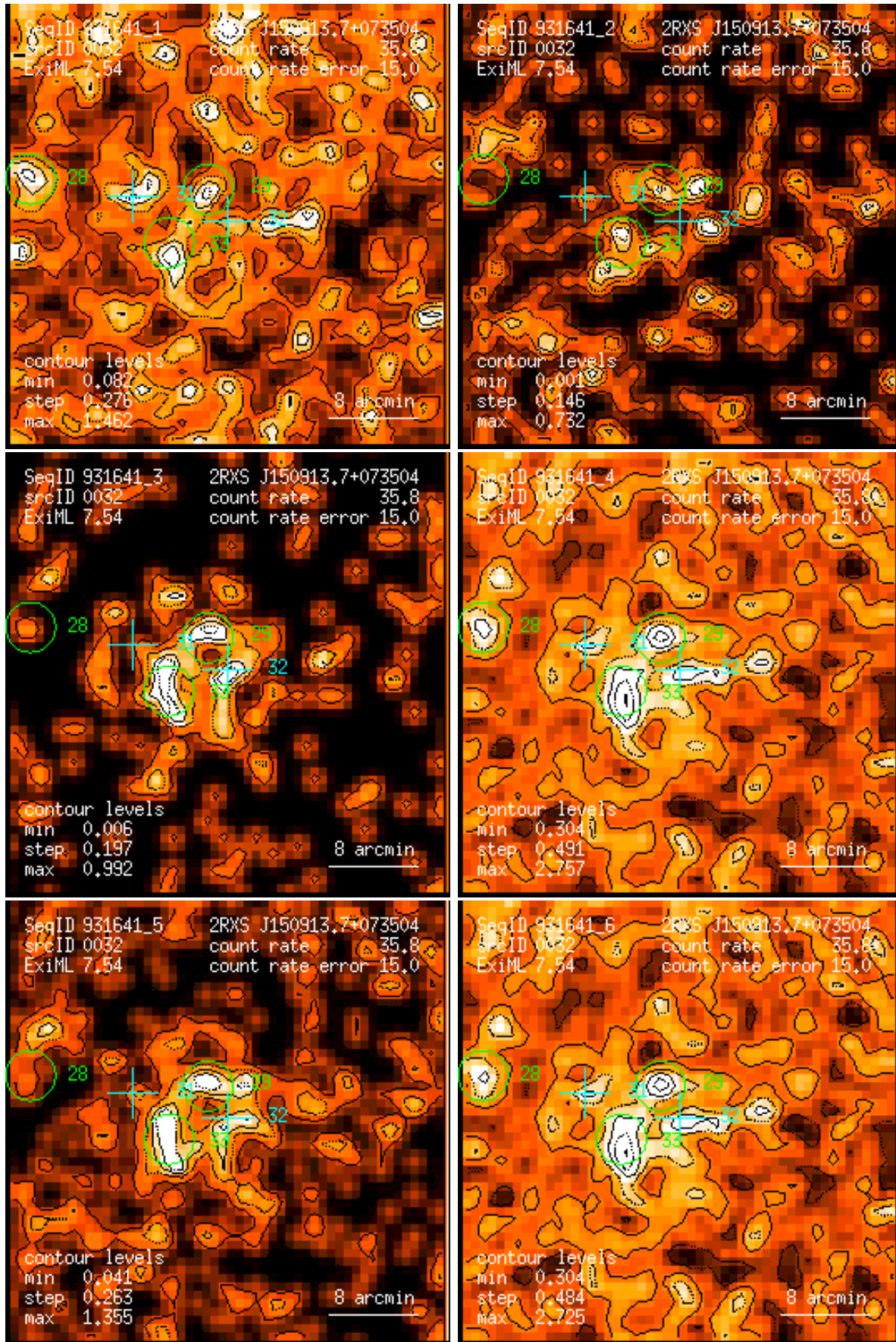
Figure 32: RASS 931641: detection 0032: band rate images, Gaussian filter: (1) PSPC channels 11 – 41, (2) 52 – 90, (3) 91 – 201, (4) 11 – 235, (5) 52 – 201, (6) 11 – 201. Broad band rates in counts/ks. Band rate contour levels in counts/ks/arcmin 2 .
