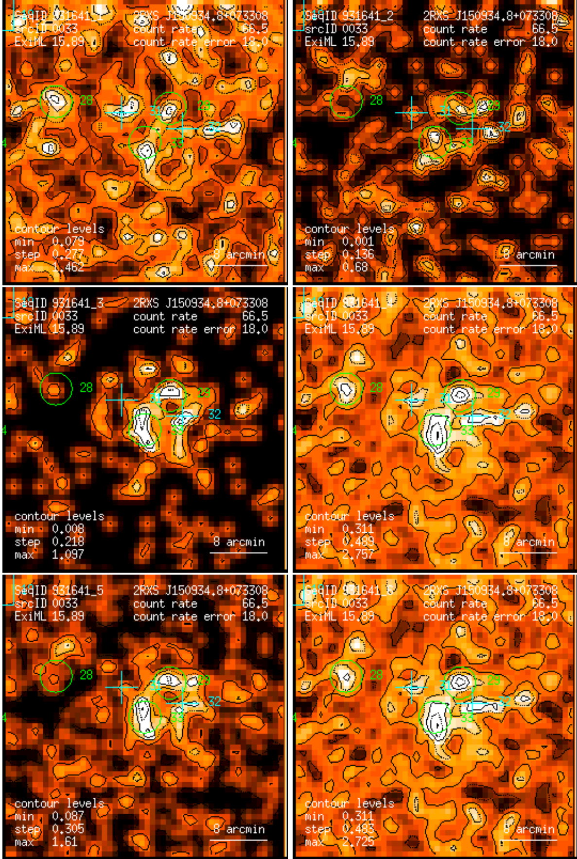
Figure 33: RASS 931641: detection 0033: band rate images, Gaussian filter: (1) PSPC channels 11 – 41, (2) 52 – 90, (3) 91 – 201, (4) 11 – 235, (5) 52 – 201, (6) 11 – 201. Broad band rates in counts/ks. Band rate contour levels in counts/ks/arcmin 2 .
