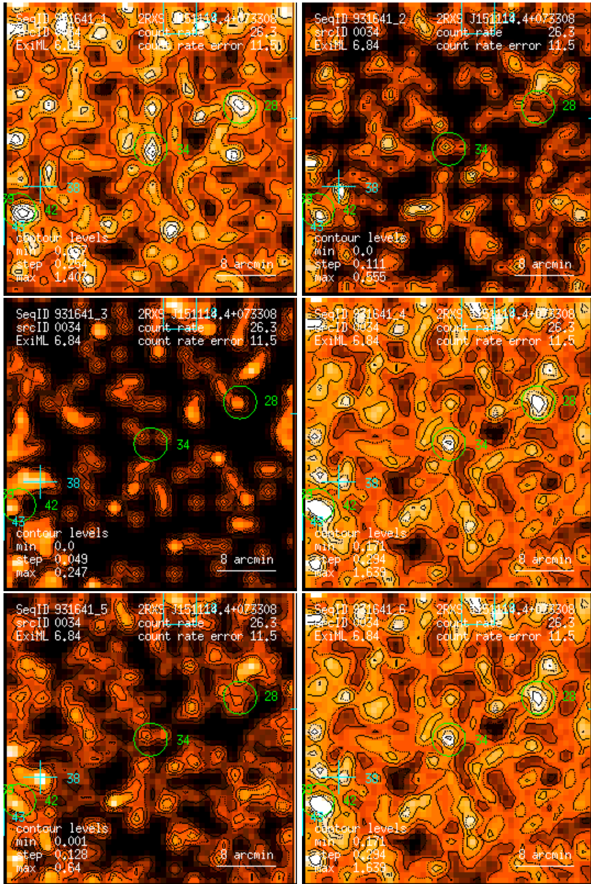
Figure 34: RASS 931641: detection 0034: band rate images, Gaussian filter: (1) PSPC channels 11 – 41, (2) 52 – 90, (3) 91 – 201, (4) 11 – 235, (5) 52 – 201, (6) 11 – 201. Broad band rates in counts/ks. Band rate contour levels in counts/ks/arcmin 2 .
