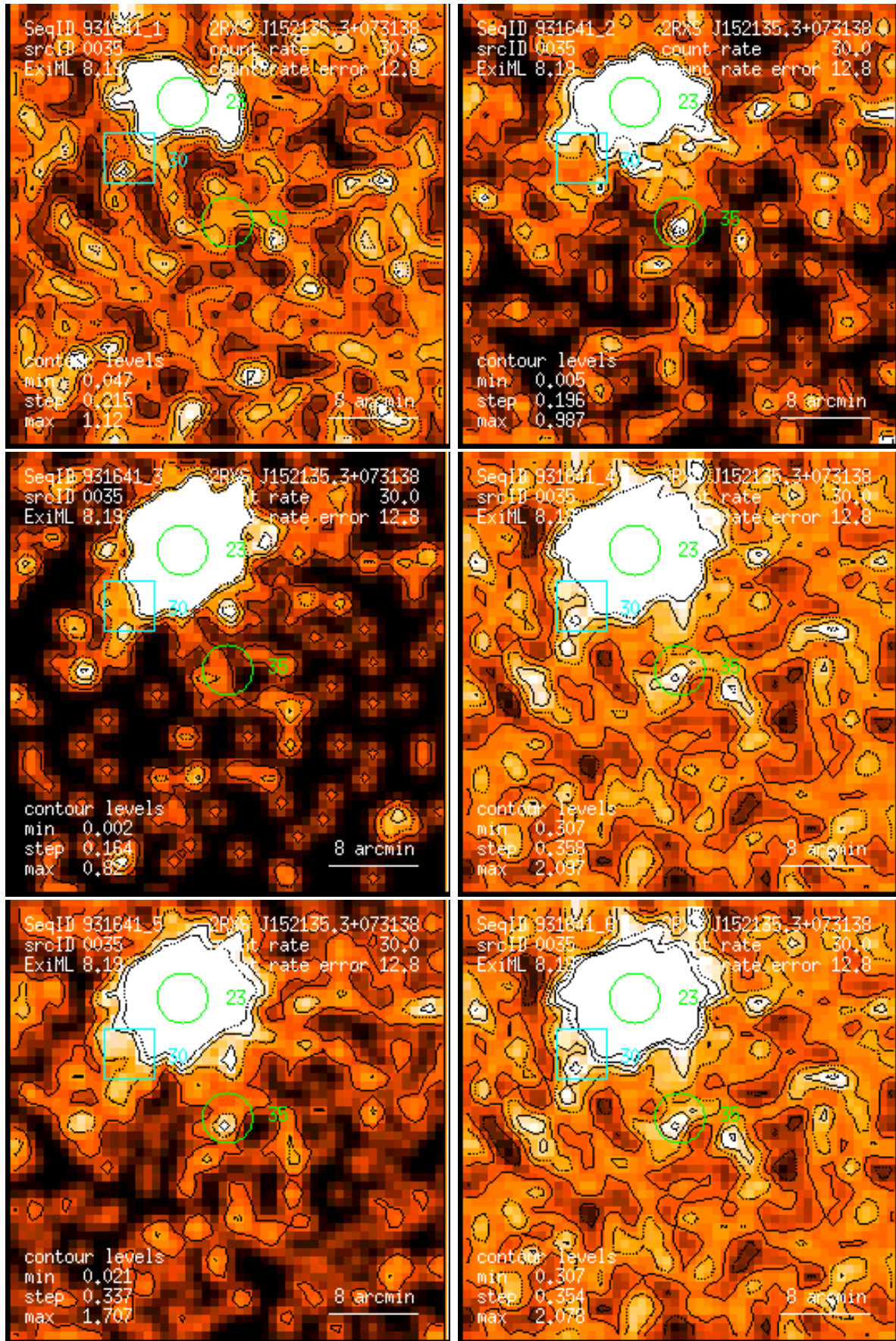
Figure 35: RASS 931641: detection 0035: band rate images, Gaussian filter: (1) PSPC channels 11 – 41, (2) 52 – 90, (3) 91 – 201, (4) 11 – 235, (5) 52 – 201, (6) 11 – 201. Broad band rates in counts/ks. Band rate contour levels in counts/ks/arcmin 2 .
