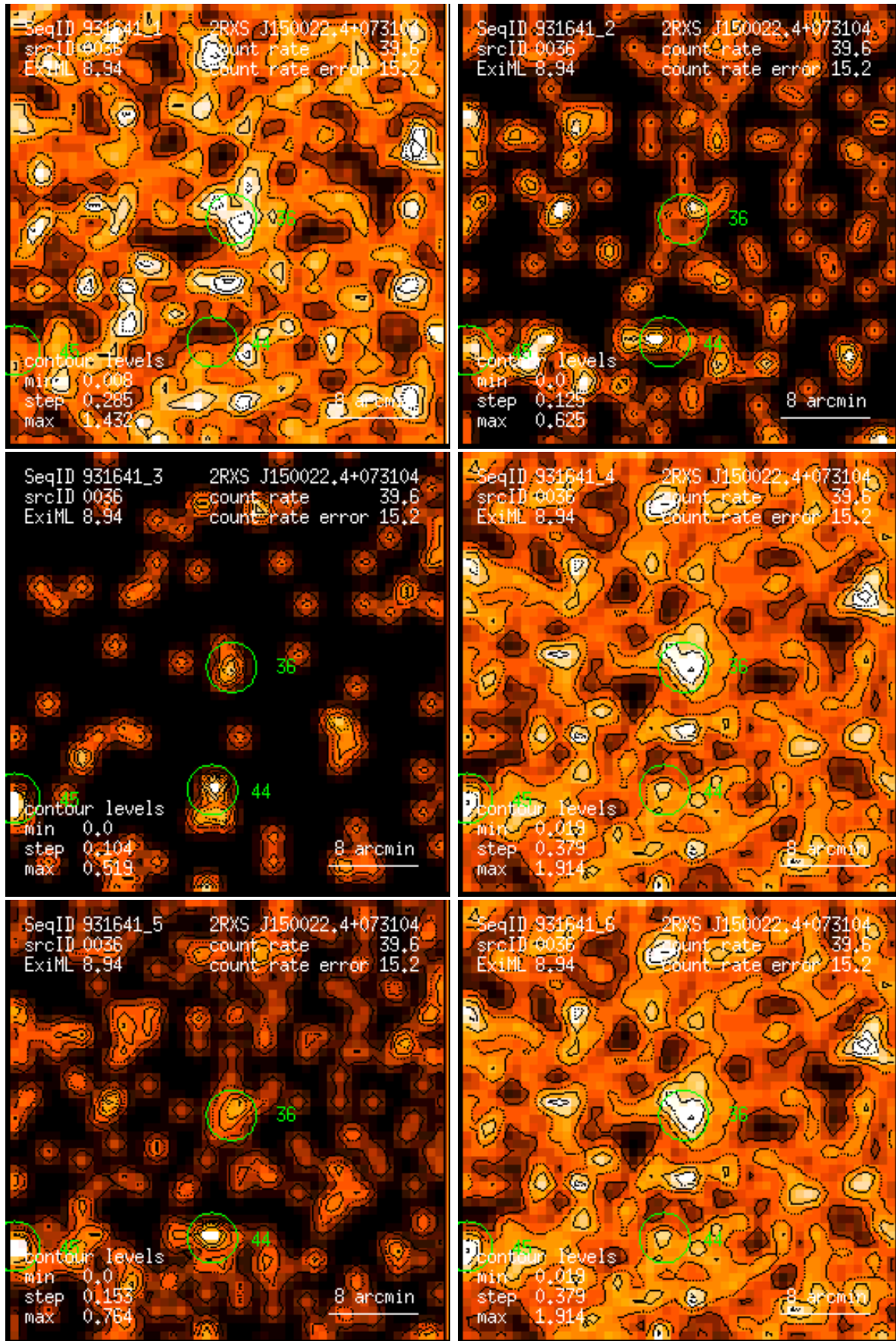
Figure 36: RASS 931641: detection 0036: band rate images, Gaussian filter: (1) PSPC channels 11 – 41, (2) 52 – 90, (3) 91 – 201, (4) 11 – 235, (5) 52 – 201, (6) 11 – 201. Broad band rates in counts/ks. Band rate contour levels in counts/ks/arcmin 2 .
