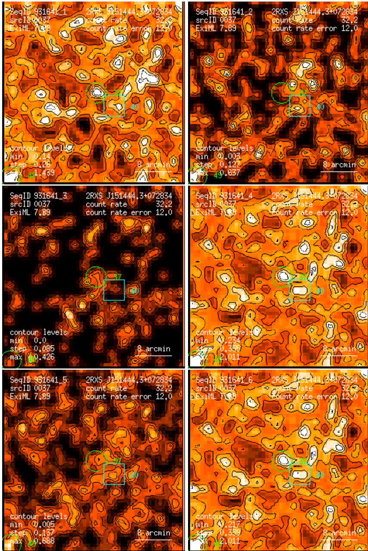
Figure 37: RASS 931641: detection 0037: band rate images, Gaussian filter: (1) PSPC channels 11 – 41, (2) 52 – 90, (3) 91 – 201, (4) 11 – 235, (5) 52 – 201, (6) 11 – 201. Broad band rates in counts/ks. Band rate contour levels in counts/ks/arcmin 2 .
