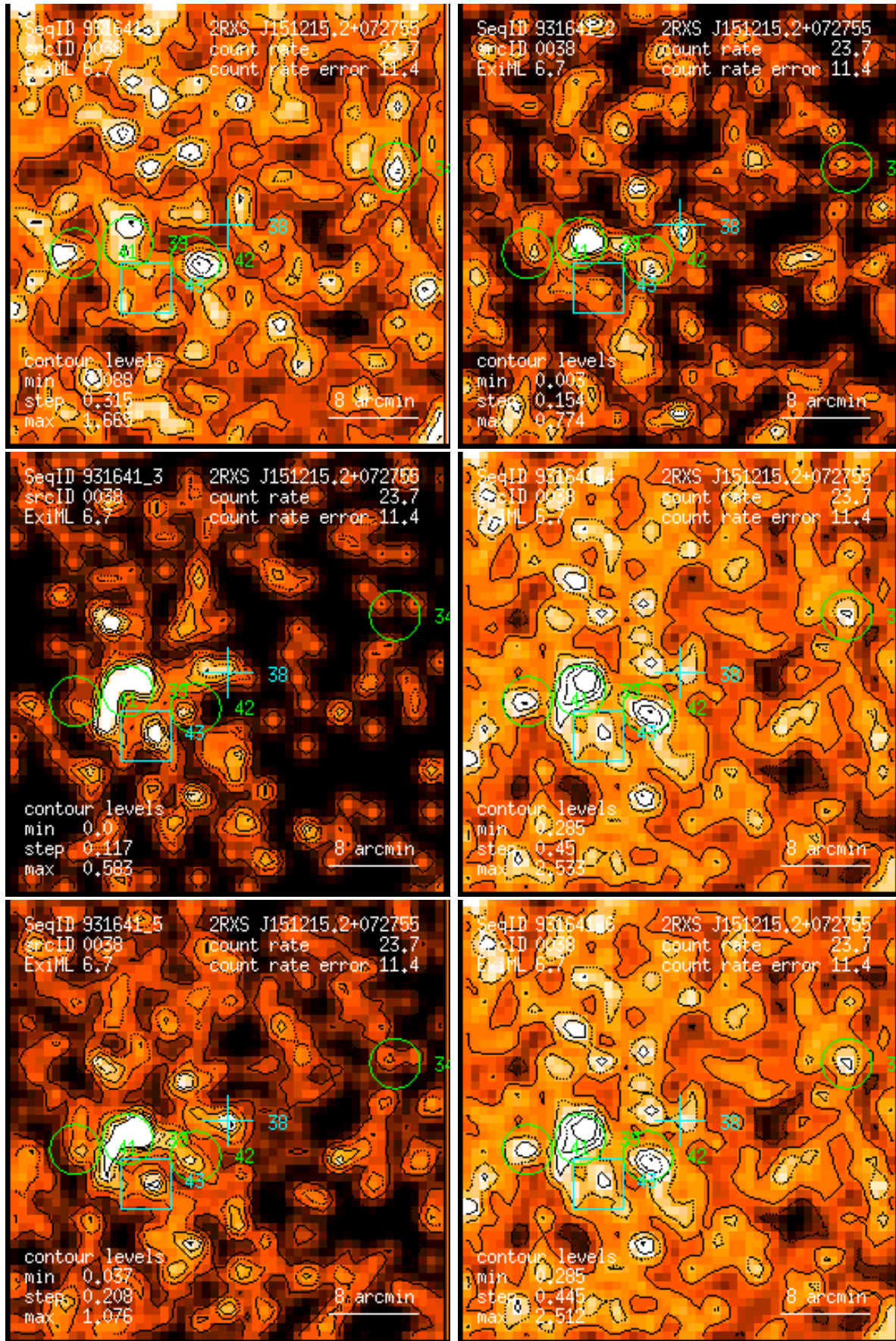
Figure 38: RASS 931641: detection 0038: band rate images, Gaussian filter: (1) PSPC channels 11 – 41, (2) 52 – 90, (3) 91 – 201, (4) 11 – 235, (5) 52 – 201, (6) 11 – 201. Broad band rates in counts/ks. Band rate contour levels in counts/ks/arcmin 2 .
