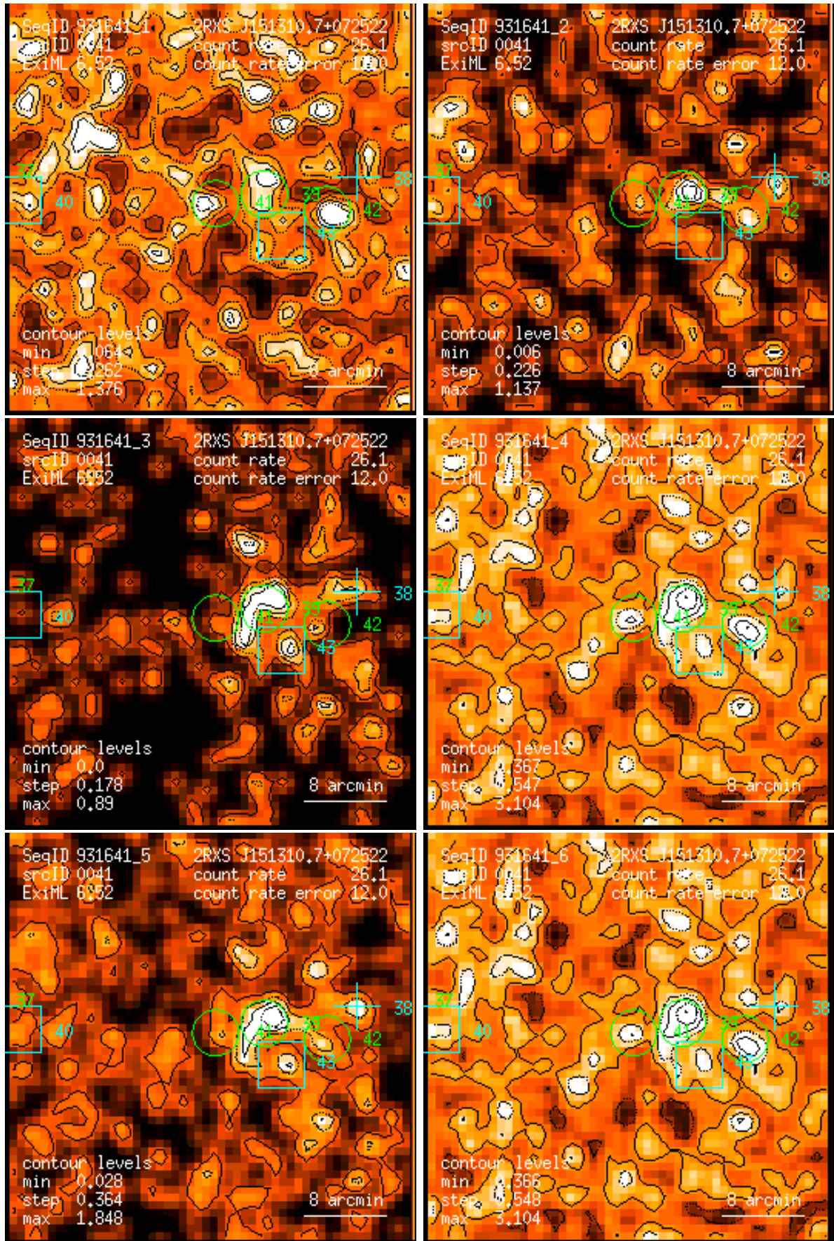
Figure 41: RASS 931641: detection 0041: band rate images, Gaussian filter: (1) PSPC channels 11 – 41, (2) 52 – 90, (3) 91 – 201, (4) 11 – 235, (5) 52 – 201, (6) 11 – 201. Broad band rates in counts/ks. Band rate contour levels in counts/ks/arcmin 2 .
