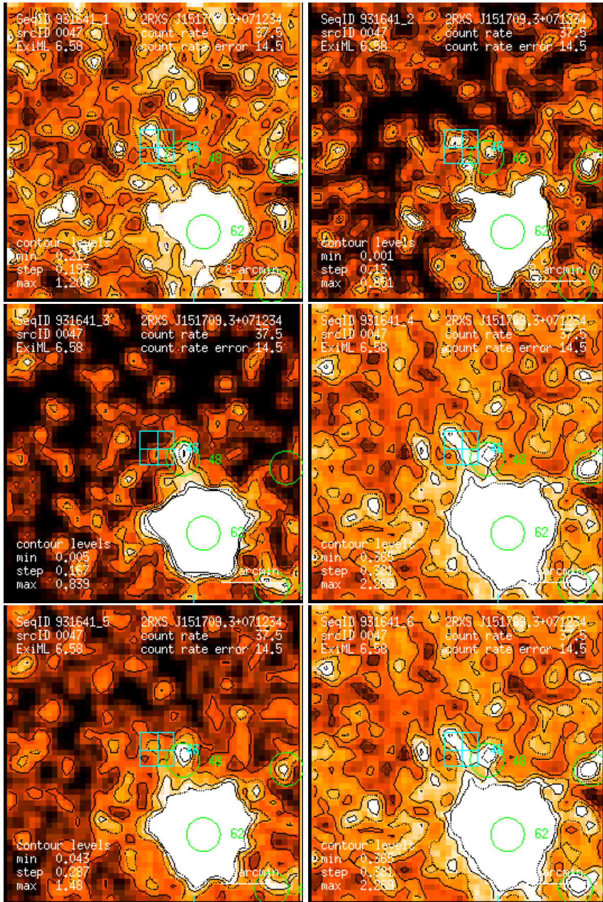
Figure 47: RASS 931641: detection 0047: band rate images, Gaussian filter: (1) PSPC channels 11 – 41, (2) 52 – 90, (3) 91 – 201, (4) 11 – 235, (5) 52 – 201, (6) 11 – 201. Broad band rates in counts/ks. Band rate contour levels in counts/ks/arcmin 2 .
