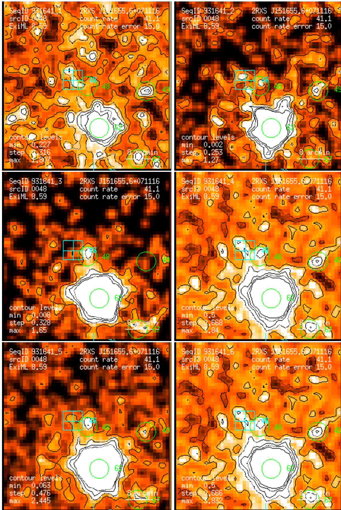
Figure 48: RASS 931641: detection 0048: band rate images, Gaussian filter: (1) PSPC channels 11 – 41, (2) 52 – 90, (3) 91 – 201, (4) 11 – 235, (5) 52 – 201, (6) 11 – 201. Broad band rates in counts/ks. Band rate contour levels in counts/ks/arcmin 2 .
