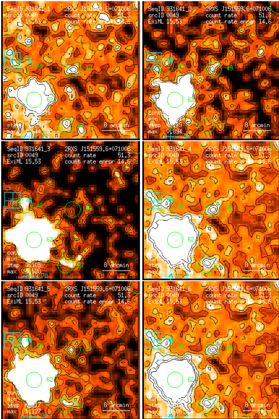
Figure 49: RASS 931641: detection 0049: band rate images, Gaussian filter: (1) PSPC channels 11 – 41, (2) 52 – 90, (3) 91 – 201, (4) 11 – 235, (5) 52 – 201, (6) 11 – 201. Broad band rates in counts/ks. Band rate contour levels in counts/ks/arcmin 2 .
