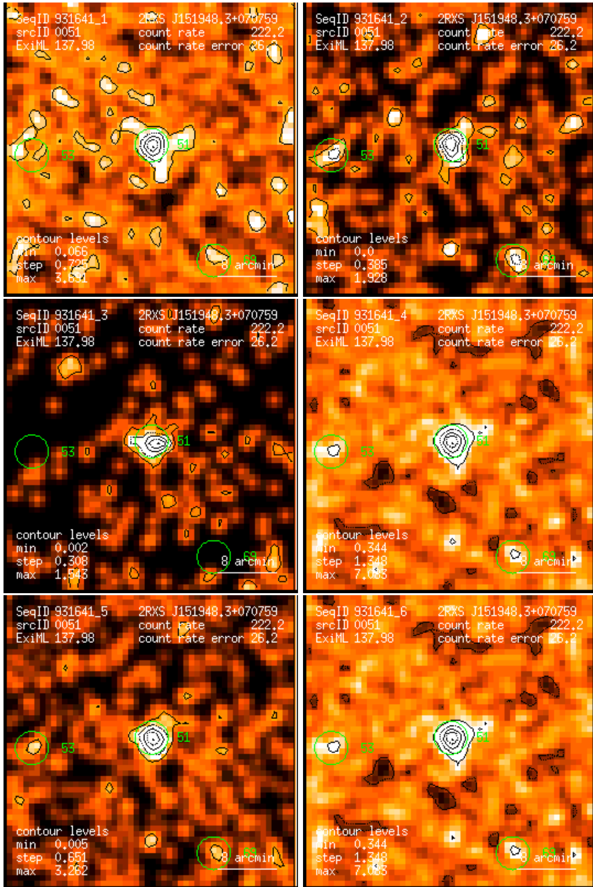
Figure 51: RASS 931641: detection 0051: band rate images, Gaussian filter: (1) PSPC channels 11 – 41, (2) 52 – 90, (3) 91 – 201, (4) 11 – 235, (5) 52 – 201, (6) 11 – 201. Broad band rates in counts/ks. Band rate contour levels in counts/ks/arcmin 2 .
