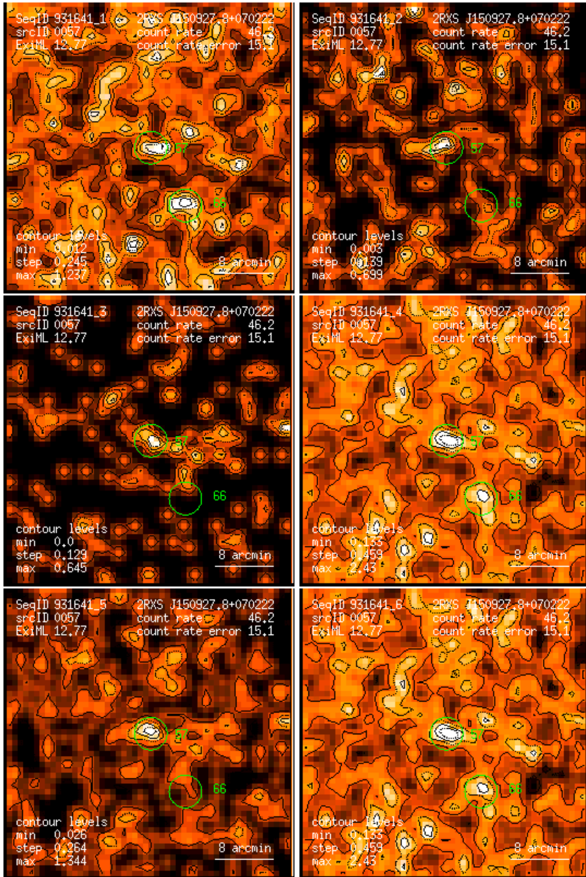
Figure 57: RASS 931641: detection 0057: band rate images, Gaussian filter: (1) PSPC channels 11 – 41, (2) 52 – 90, (3) 91 – 201, (4) 11 – 235, (5) 52 – 201, (6) 11 – 201. Broad band rates in counts/ks. Band rate contour levels in counts/ks/arcmin 2 .
