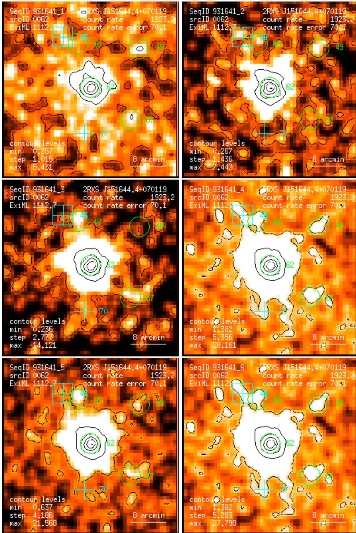
Figure 62: RASS 931641: detection 0062: band rate images, Gaussian filter: (1) PSPC channels 11 – 41, (2) 52 – 90, (3) 91 – 201, (4) 11 – 235, (5) 52 – 201, (6) 11 – 201. Broad band rates in counts/ks. Band rate contour levels in counts/ks/arcmin 2 .
