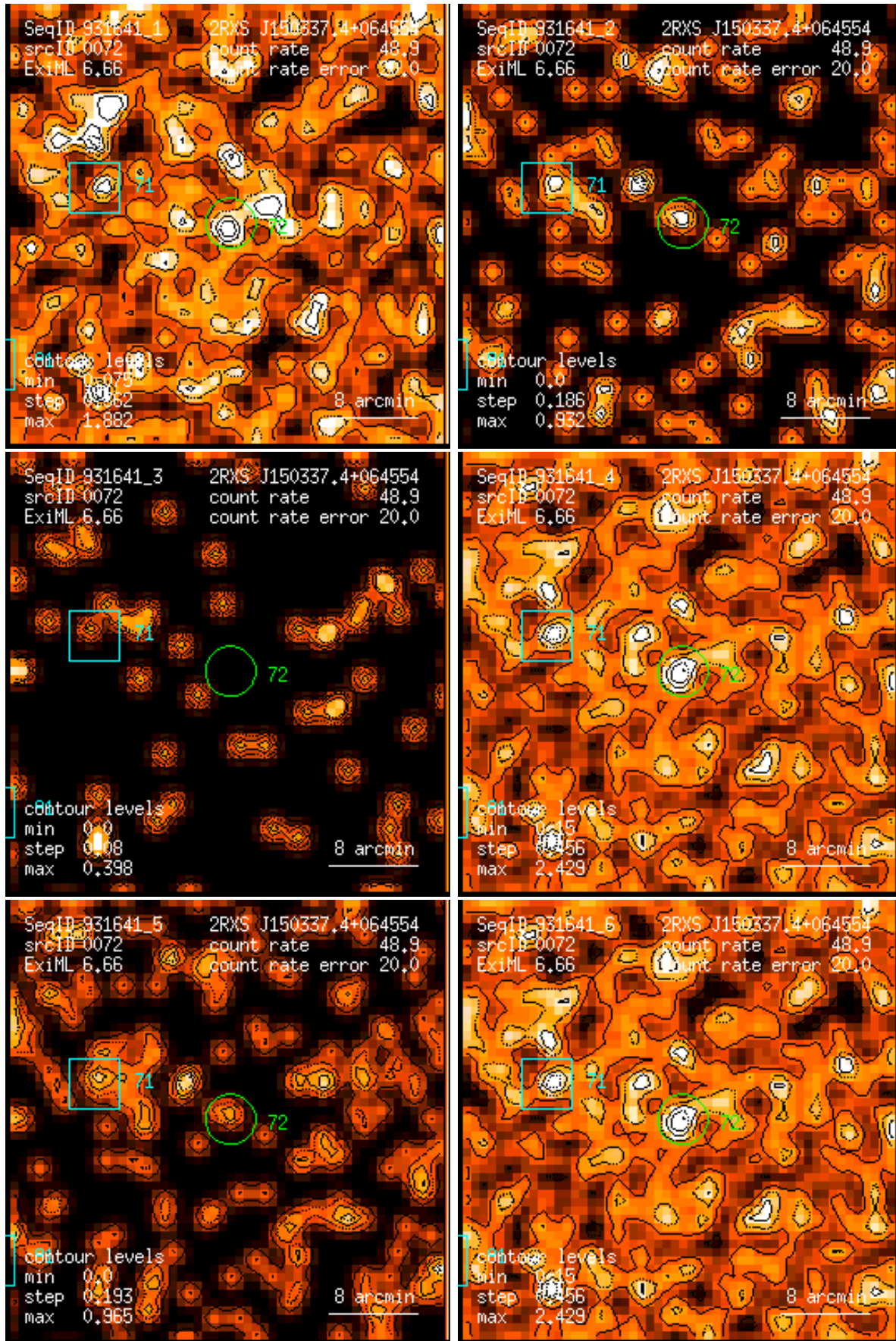
Figure 72: RASS 931641: detection 0072: band rate images, Gaussian filter: (1) PSPC channels 11 – 41, (2) 52 – 90, (3) 91 – 201, (4) 11 – 235, (5) 52 – 201, (6) 11 – 201. Broad band rates in counts/ks. Band rate contour levels in counts/ks/arcmin 2 .
